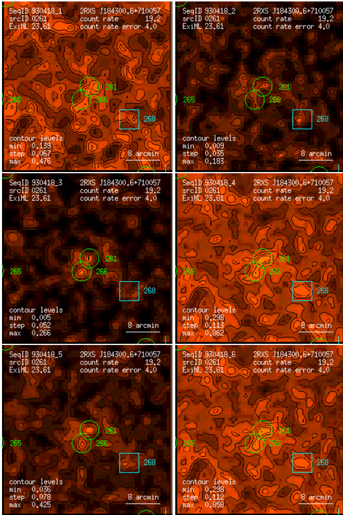
Figure 261: RASS 930418: detection 0261: band rate images, Gaussian filter: (1) PSPC channels 11 – 41, (2) 52 – 90, (3) 91 – 201, (4) 11 – 235, (5) 52 – 201, (6) 11 – 201. Broad band rates in counts/ks. Band rate contour levels in counts/ks/arcmin 2 .
