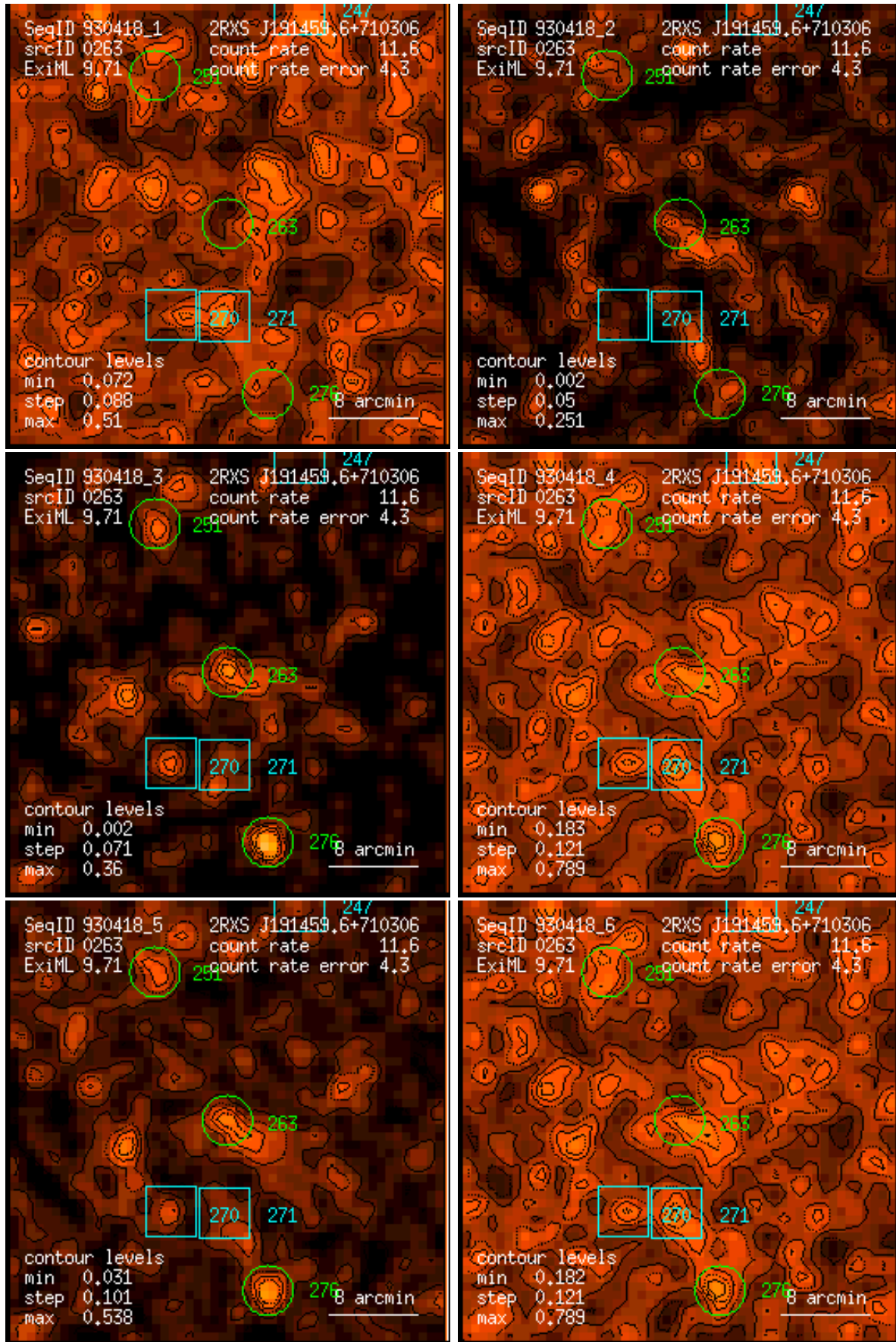
Figure 263: RASS 930418: detection 0263: band rate images, Gaussian filter: (1) PSPC channels 11 – 41, (2) 52 – 90, (3) 91 – 201, (4) 11 – 235, (5) 52 – 201, (6) 11 – 201. Broad band rates in counts/ks. Band rate contour levels in counts/ks/arcmin 2 .
