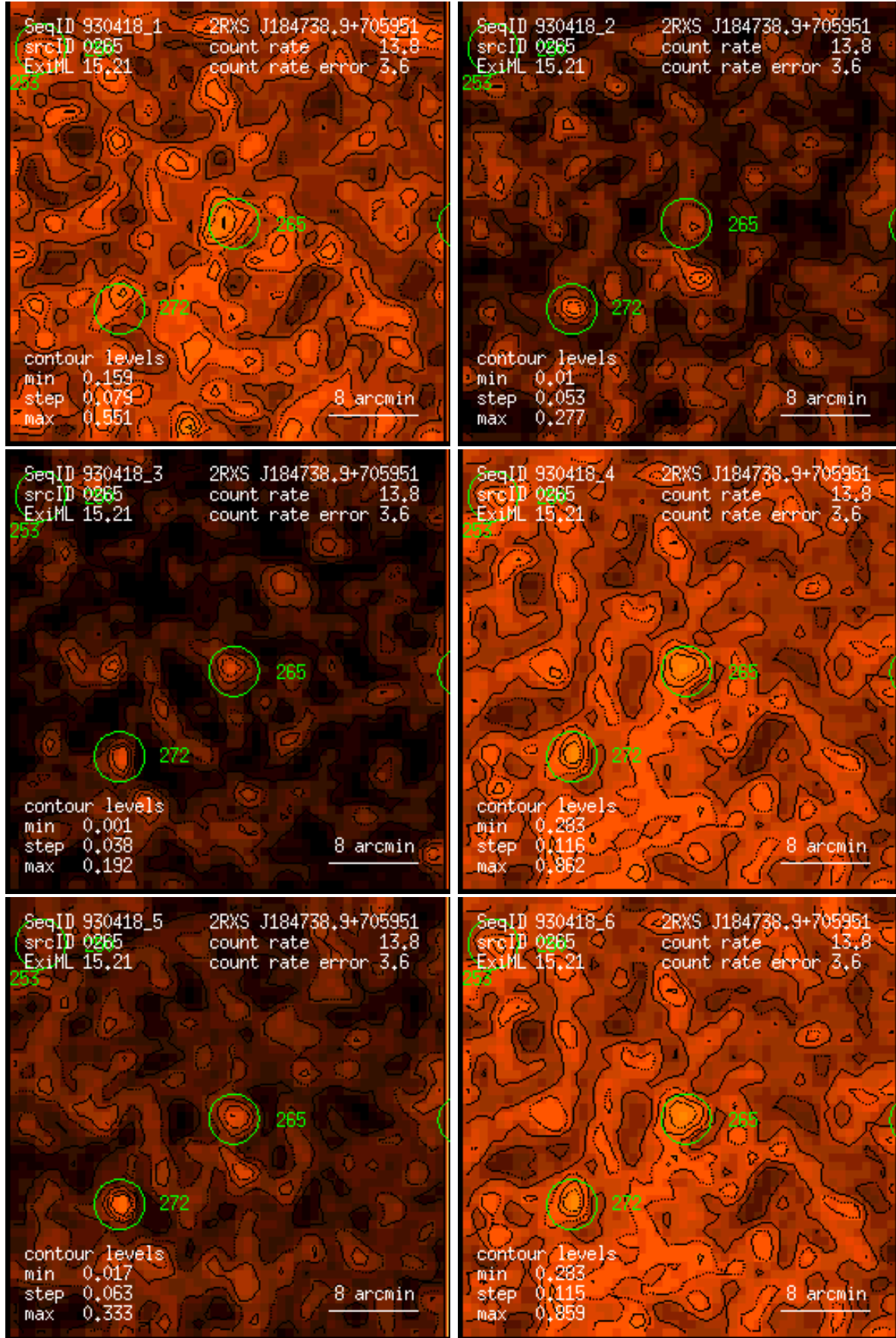
Figure 265: RASS 930418: detection 0265: band rate images, Gaussian filter: (1) PSPC channels 11 – 41, (2) 52 – 90, (3) 91 – 201, (4) 11 – 235, (5) 52 – 201, (6) 11 – 201. Broad band rates in counts/ks. Band rate contour levels in counts/ks/arcmin 2 .
