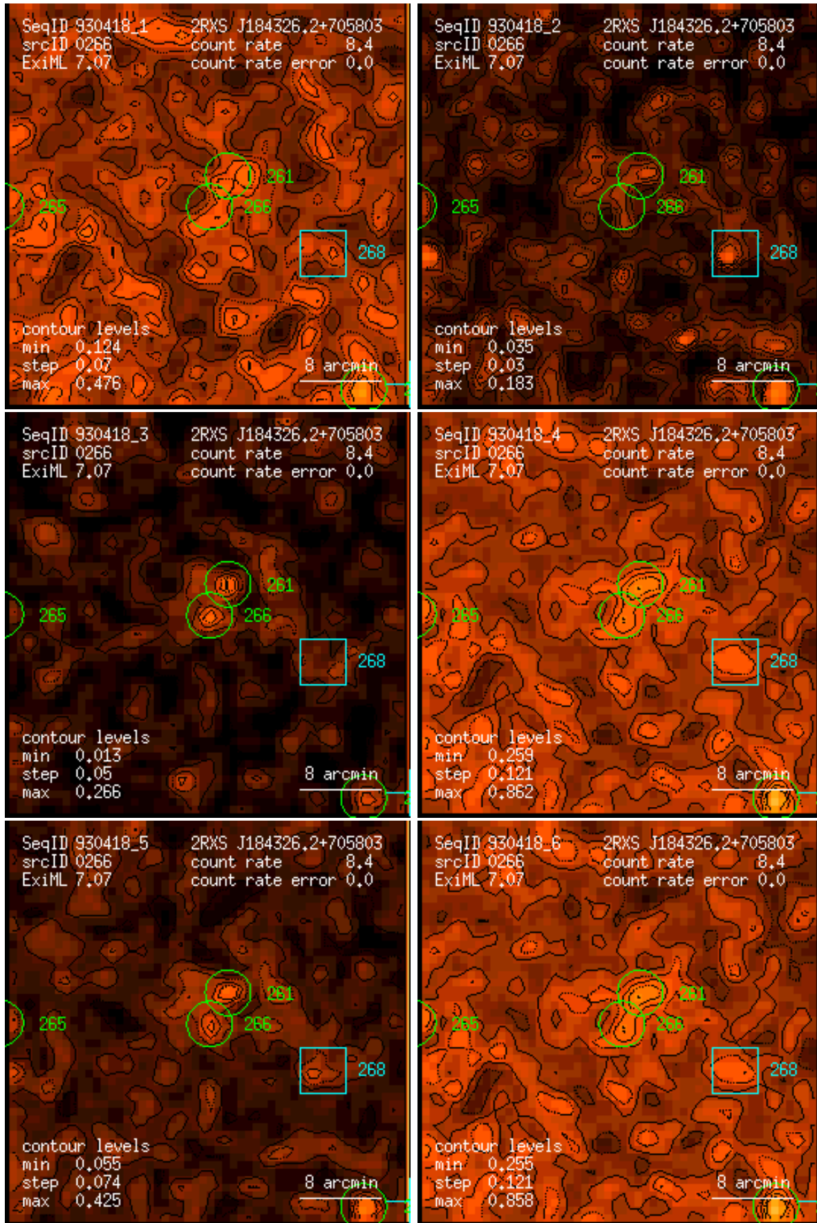
Figure 266: RASS 930418: detection 0266: band rate images, Gaussian filter: (1) PSPC channels 11 – 41, (2) 52 – 90, (3) 91 – 201, (4) 11 – 235, (5) 52 – 201, (6) 11 – 201. Broad band rates in counts/ks. Band rate contour levels in counts/ks/arcmin 2 .
