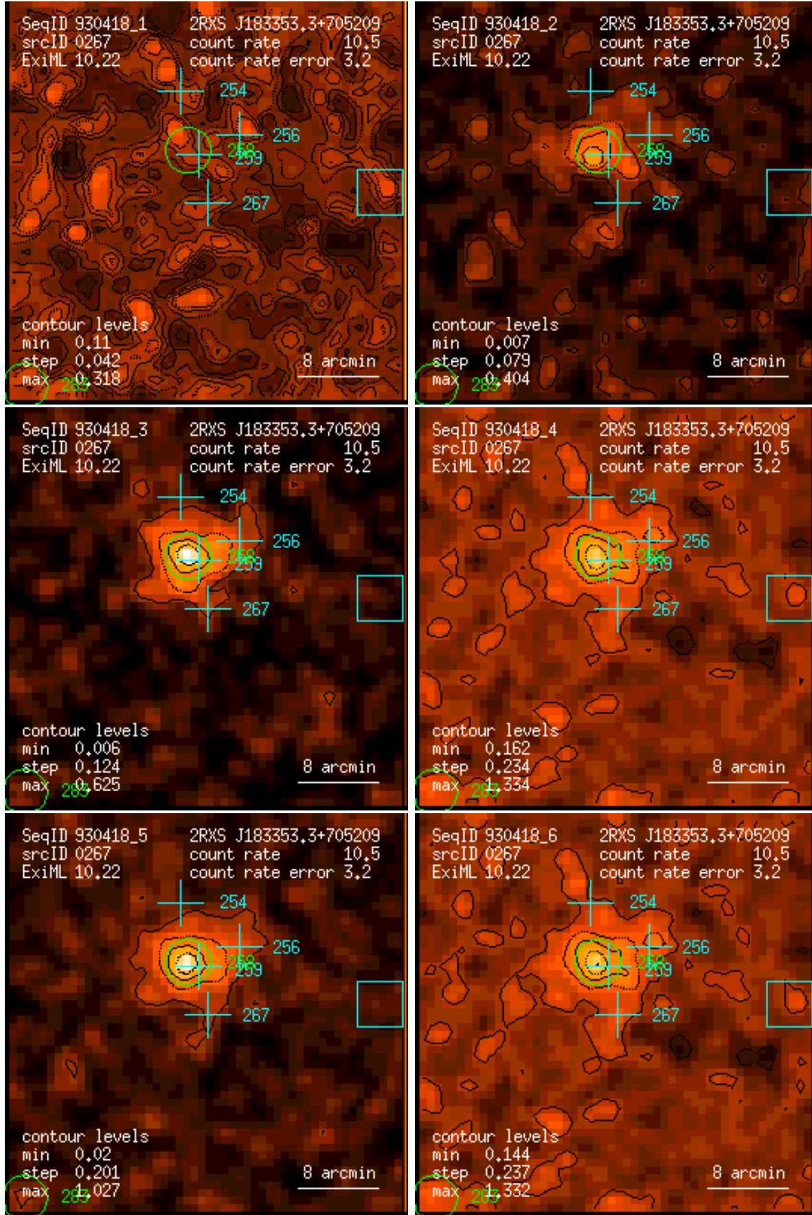
Figure 267: RASS 930418: detection 0267: band rate images, Gaussian filter: (1) PSPC channels 11 – 41, (2) 52 – 90, (3) 91 – 201, (4) 11 – 235, (5) 52 – 201, (6) 11 – 201. Broad band rates in counts/ks. Band rate contour levels in counts/ks/arcmin 2 .
