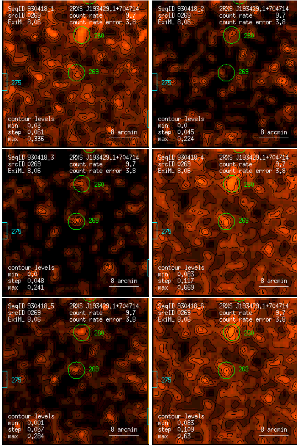
Figure 269: RASS 930418: detection 0269: band rate images, Gaussian filter: (1) PSPC channels 11 – 41, (2) 52 – 90, (3) 91 – 201, (4) 11 – 235, (5) 52 – 201, (6) 11 – 201. Broad band rates in counts/ks. Band rate contour levels in counts/ks/arcmin 2 .
