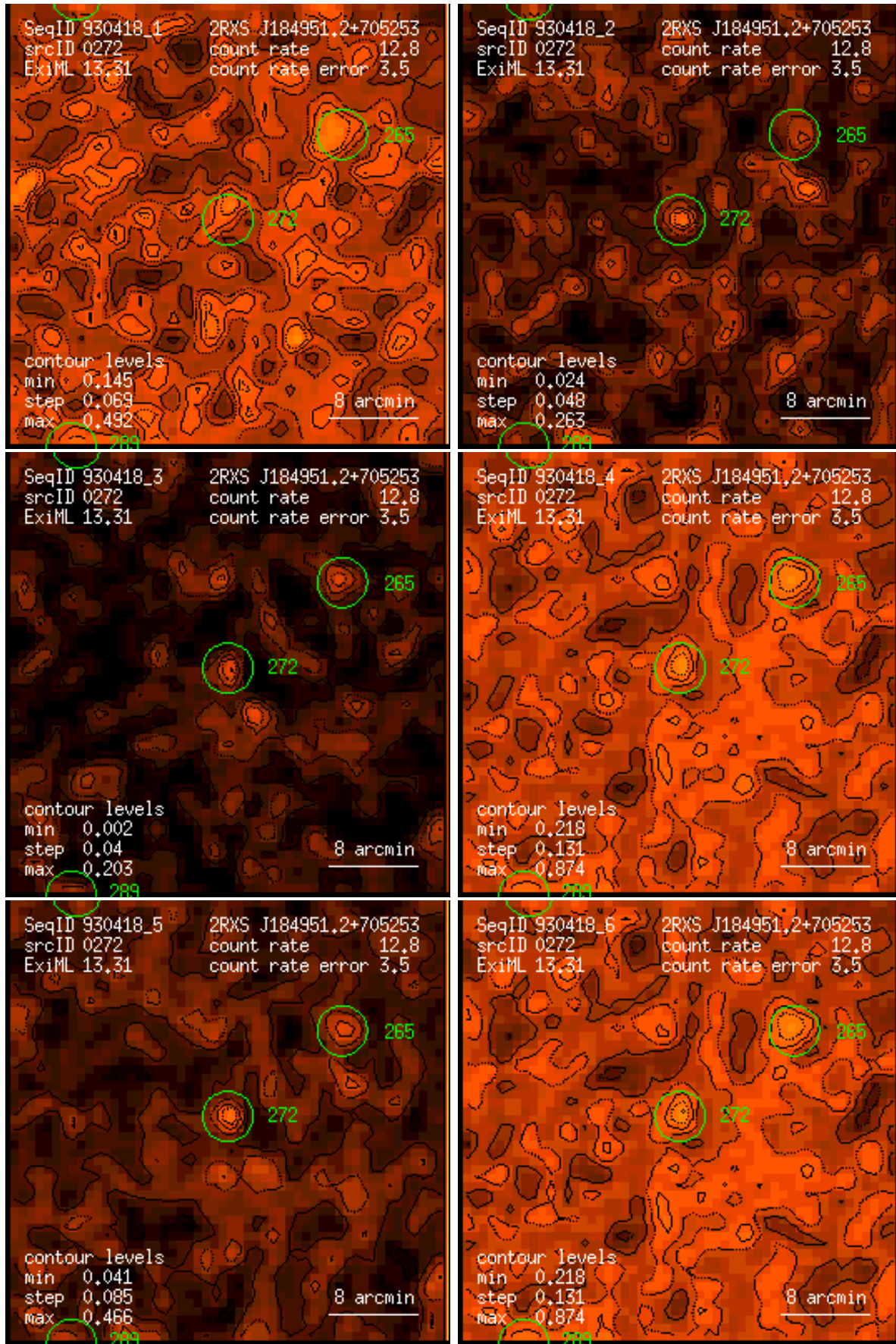
Figure 272: RASS 930418: detection 0272: band rate images, Gaussian filter: (1) PSPC channels 11 – 41, (2) 52 – 90, (3) 91 – 201, (4) 11 – 235, (5) 52 – 201, (6) 11 – 201. Broad band rates in counts/ks. Band rate contour levels in counts/ks/arcmin 2 .
