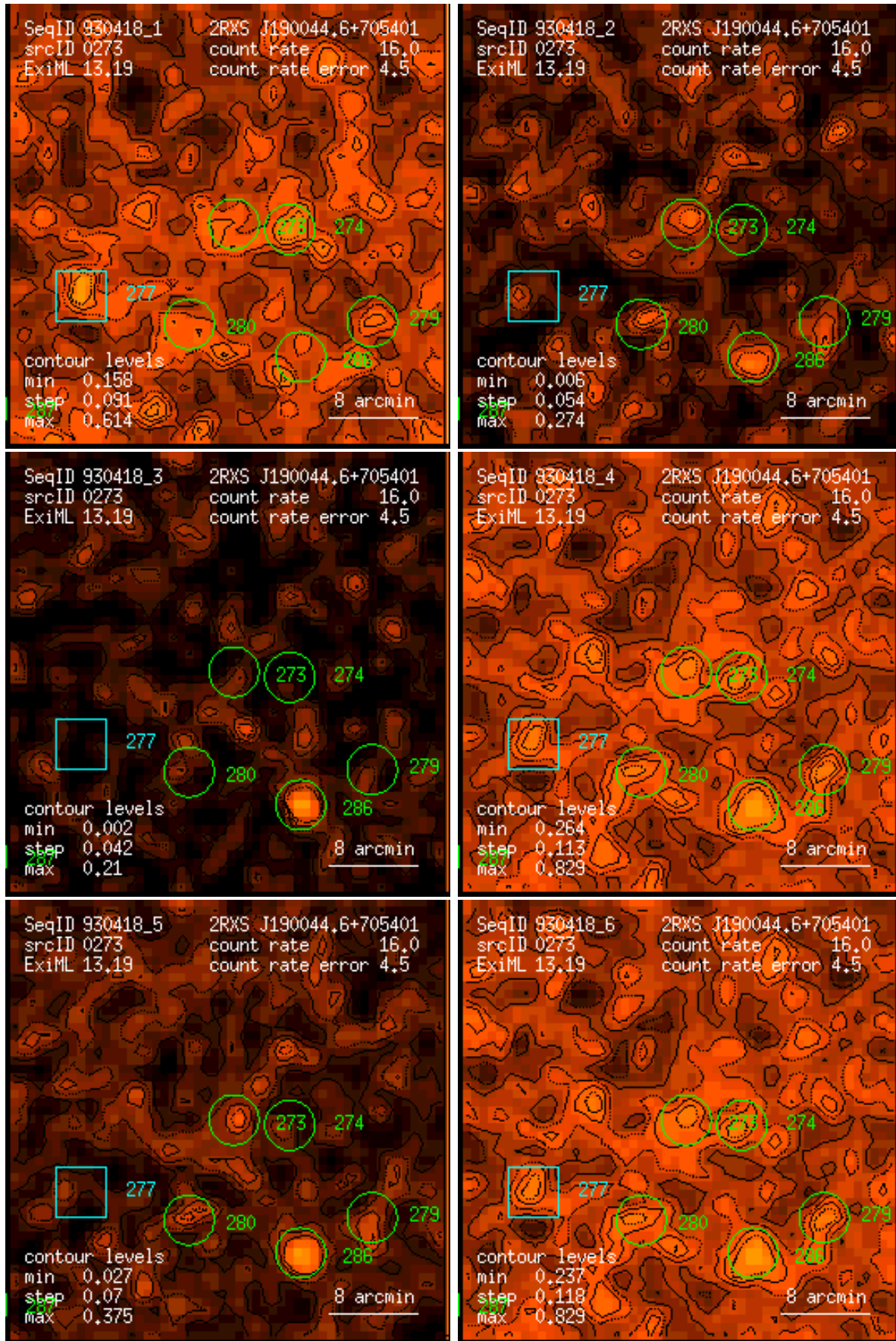
Figure 273: RASS 930418: detection 0273: band rate images, Gaussian filter: (1) PSPC channels 11 – 41, (2) 52 – 90, (3) 91 – 201, (4) 11 – 235, (5) 52 – 201, (6) 11 – 201. Broad band rates in counts/ks. Band rate contour levels in counts/ks/arcmin 2 .
