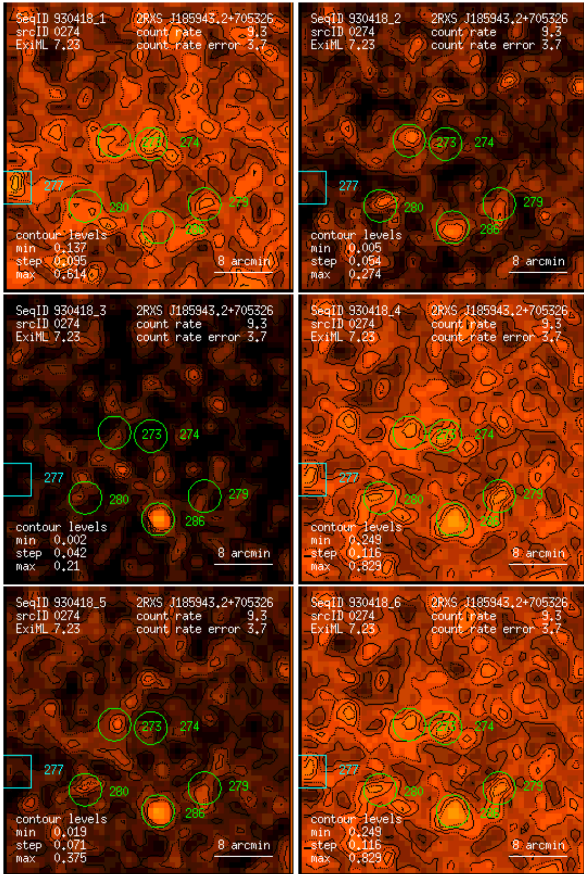
Figure 274: RASS 930418: detection 0274: band rate images, Gaussian filter: (1) PSPC channels 11 – 41, (2) 52 – 90, (3) 91 – 201, (4) 11 – 235, (5) 52 – 201, (6) 11 – 201. Broad band rates in counts/ks. Band rate contour levels in counts/ks/arcmin 2 .
