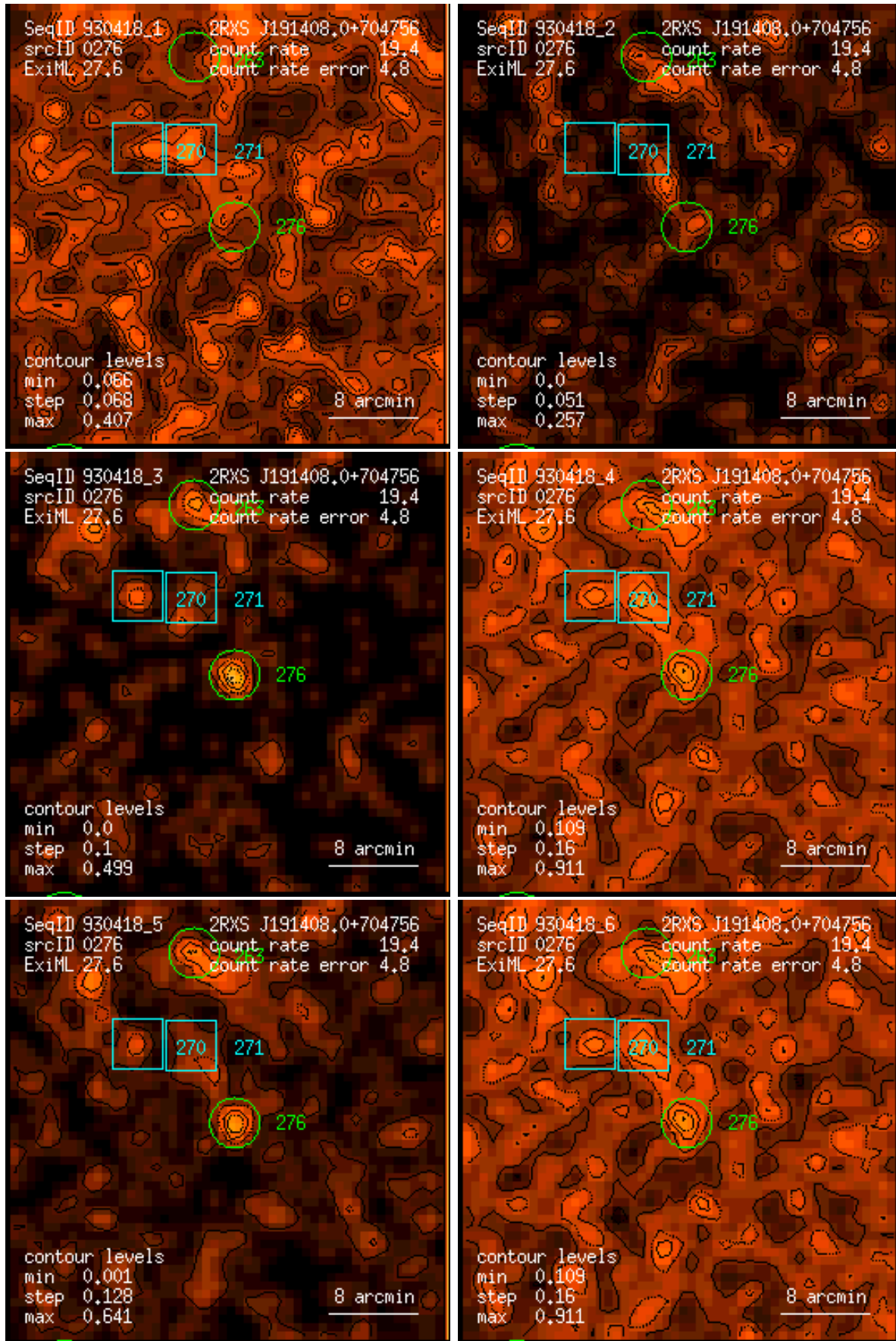
Figure 276: RASS 930418: detection 0276: band rate images, Gaussian filter: (1) PSPC channels 11 – 41, (2) 52 – 90, (3) 91 – 201, (4) 11 – 235, (5) 52 – 201, (6) 11 – 201. Broad band rates in counts/ks. Band rate contour levels in counts/ks/arcmin 2 .
