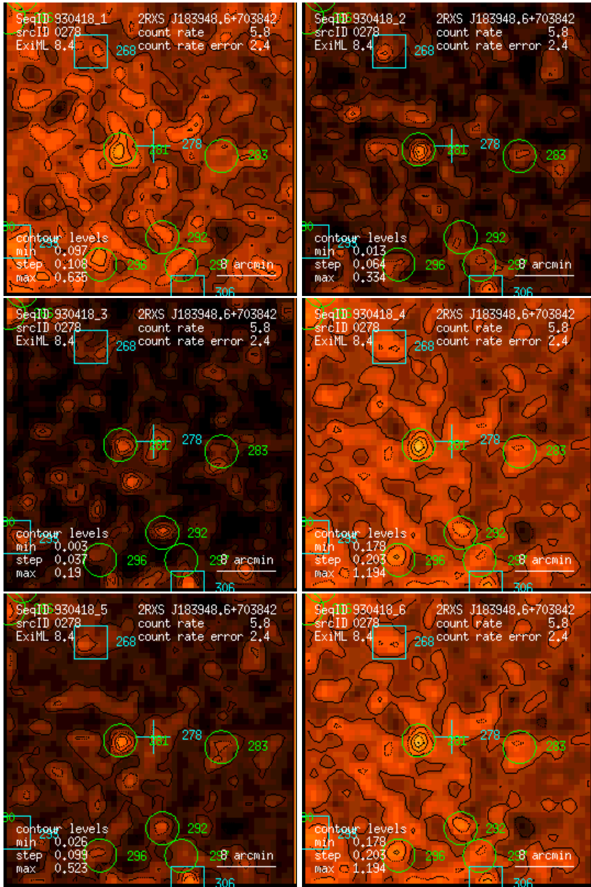
Figure 278: RASS 930418: detection 0278: band rate images, Gaussian filter: (1) PSPC channels 11 – 41, (2) 52 – 90, (3) 91 – 201, (4) 11 – 235, (5) 52 – 201, (6) 11 – 201. Broad band rates in counts/ks. Band rate contour levels in counts/ks/arcmin 2 .
