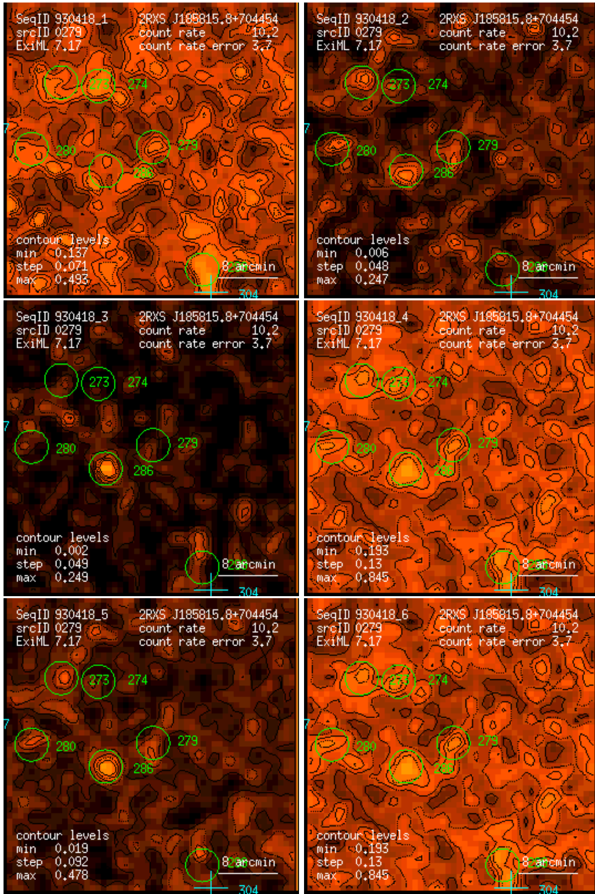
Figure 279: RASS 930418: detection 0279: band rate images, Gaussian filter: (1) PSPC channels 11 – 41, (2) 52 – 90, (3) 91 – 201, (4) 11 – 235, (5) 52 – 201, (6) 11 – 201. Broad band rates in counts/ks. Band rate contour levels in counts/ks/arcmin 2 .
