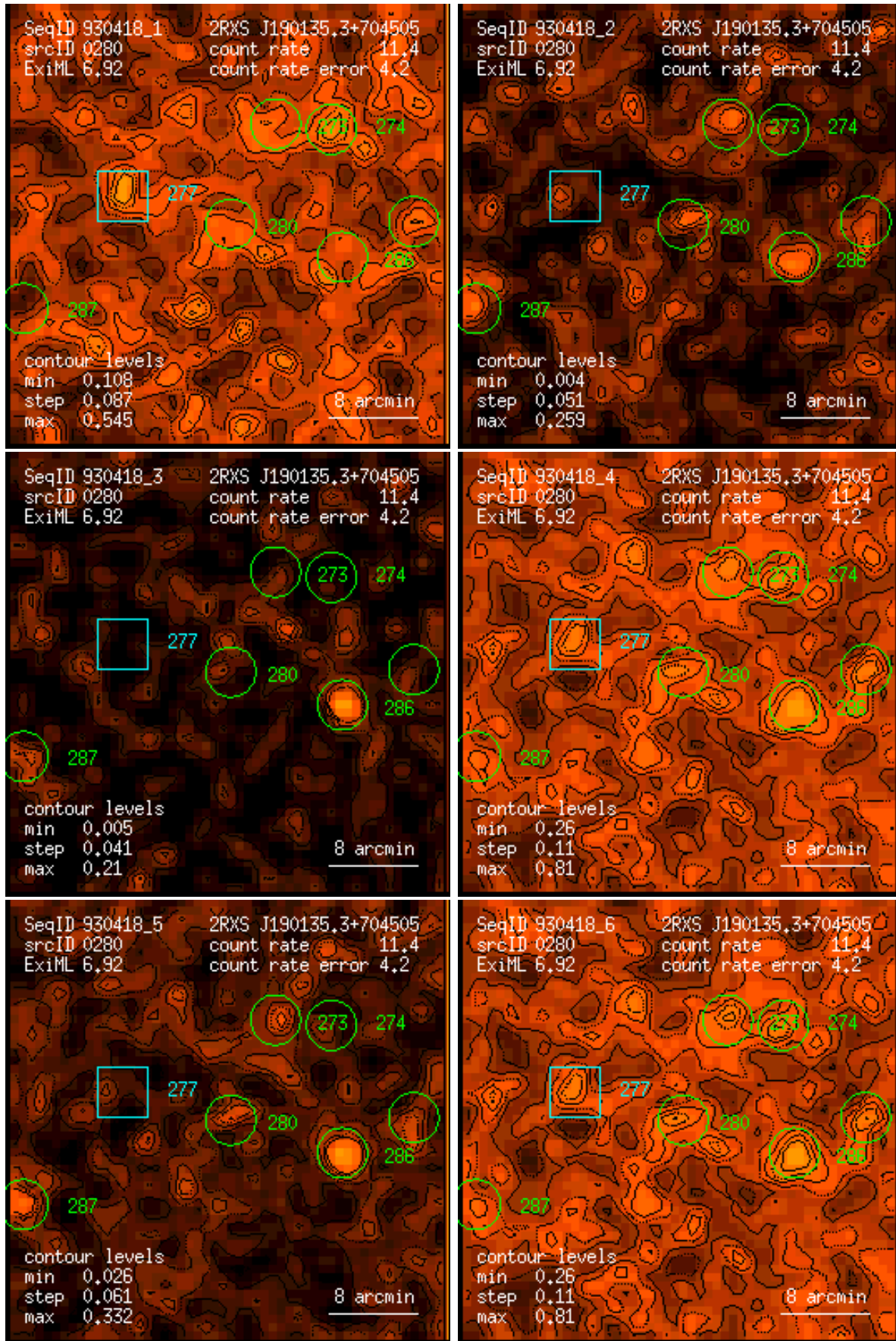
Figure 280: RASS 930418: detection 0280: band rate images, Gaussian filter: (1) PSPC channels 11 – 41, (2) 52 – 90, (3) 91 – 201, (4) 11 – 235, (5) 52 – 201, (6) 11 – 201. Broad band rates in counts/ks. Band rate contour levels in counts/ks/arcmin 2 .
