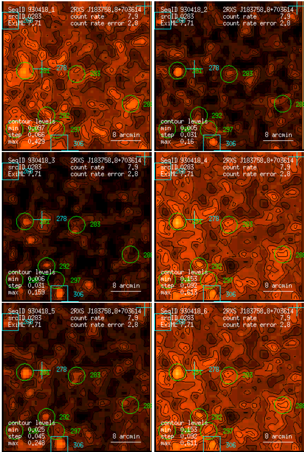
Figure 283: RASS 930418: detection 0283: band rate images, Gaussian filter: (1) PSPC channels 11 – 41, (2) 52 – 90, (3) 91 – 201, (4) 11 – 235, (5) 52 – 201, (6) 11 – 201. Broad band rates in counts/ks. Band rate contour levels in counts/ks/arcmin 2 .
