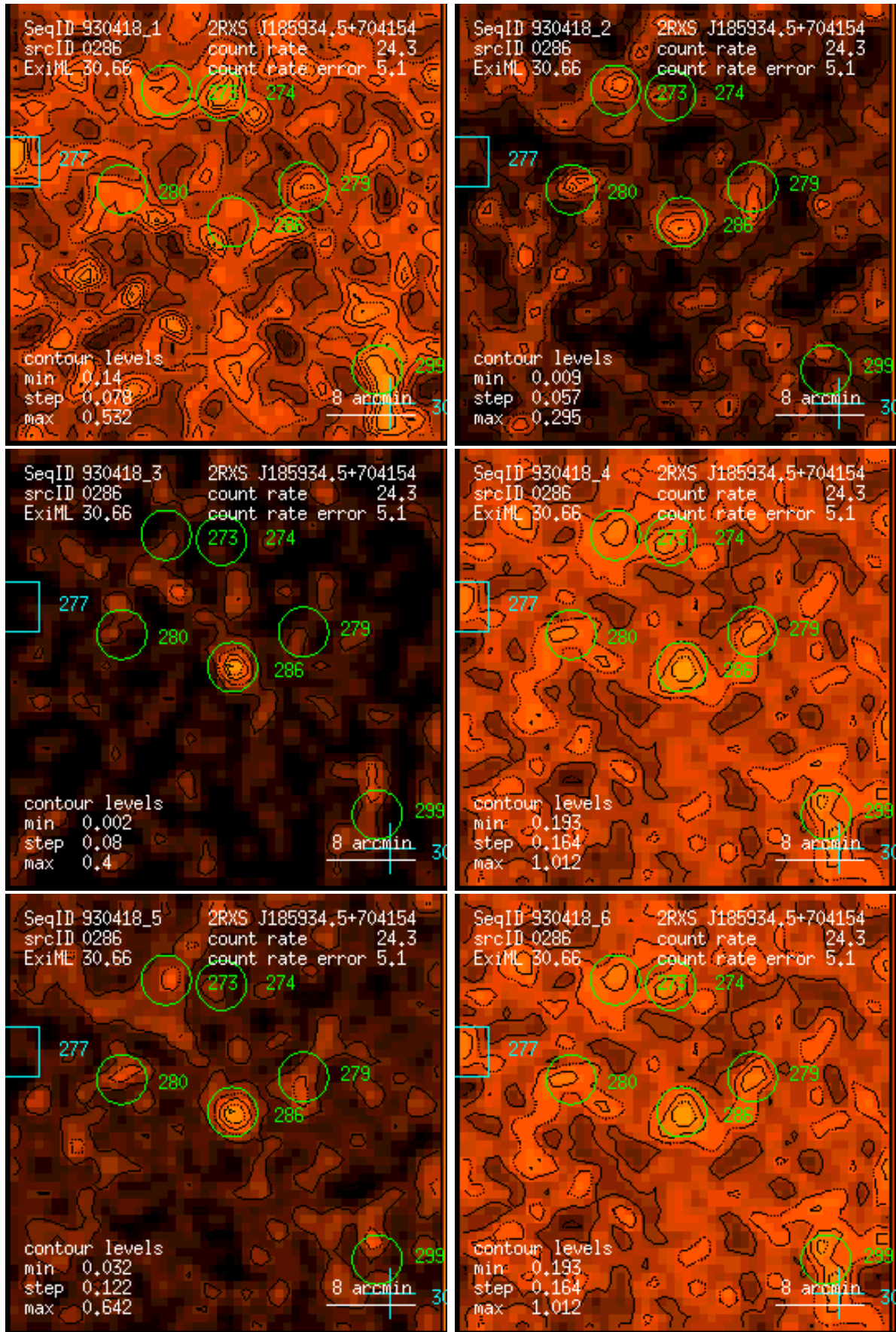
Figure 286: RASS 930418: detection 0286: band rate images, Gaussian filter: (1) PSPC channels 11 – 41, (2) 52 – 90, (3) 91 – 201, (4) 11 – 235, (5) 52 – 201, (6) 11 – 201. Broad band rates in counts/ks. Band rate contour levels in counts/ks/arcmin 2 .
