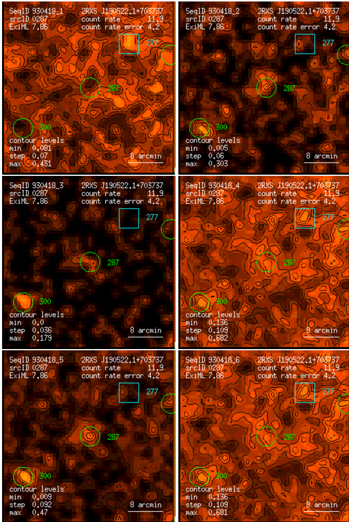
Figure 287: RASS 930418: detection 0287: band rate images, Gaussian filter: (1) PSPC channels 11 – 41, (2) 52 – 90, (3) 91 – 201, (4) 11 – 235, (5) 52 – 201, (6) 11 – 201. Broad band rates in counts/ks. Band rate contour levels in counts/ks/arcmin 2 .
