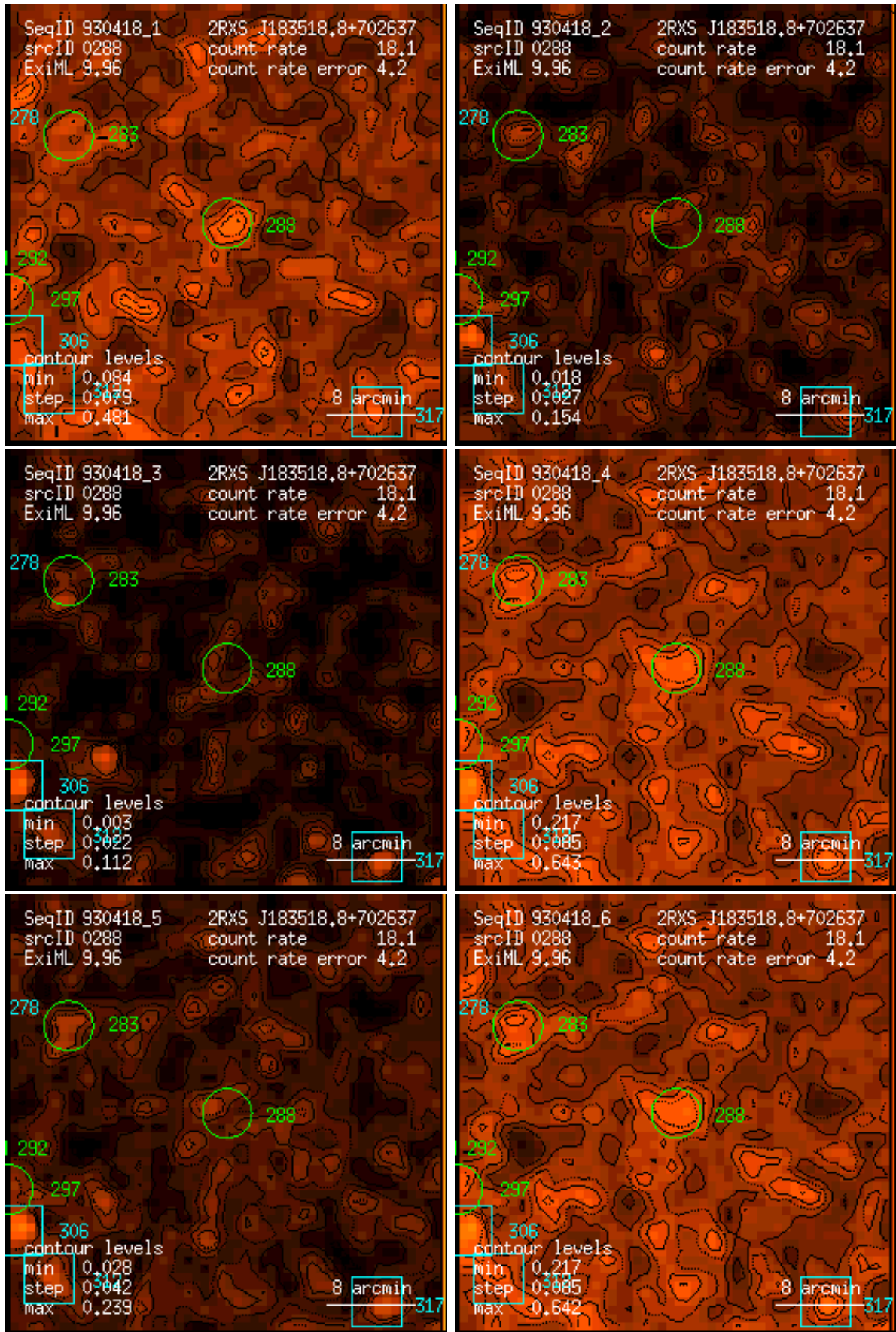
Figure 288: RASS 930418: detection 0288: band rate images, Gaussian filter: (1) PSPC channels 11 – 41, (2) 52 – 90, (3) 91 – 201, (4) 11 – 235, (5) 52 – 201, (6) 11 – 201. Broad band rates in counts/ks. Band rate contour levels in counts/ks/arcmin 2 .
