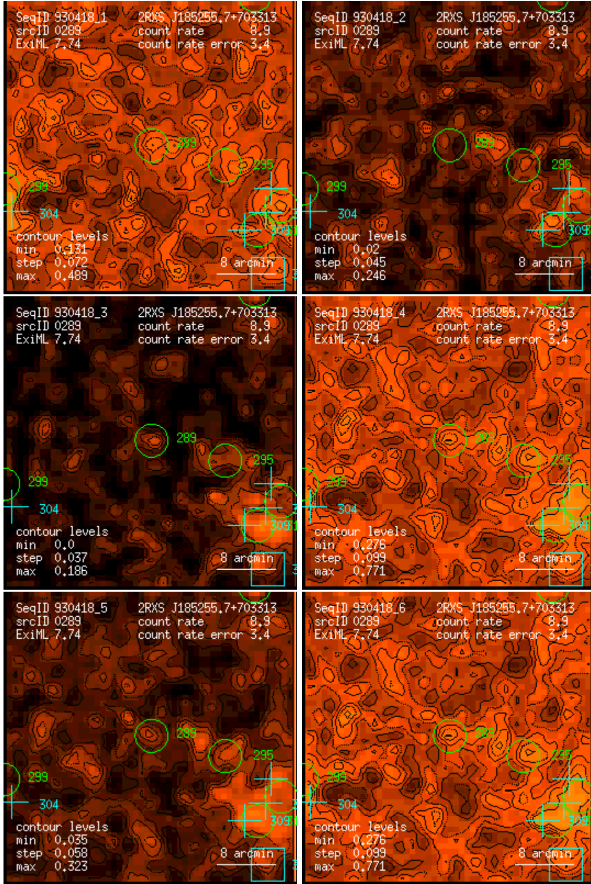
Figure 289: RASS 930418: detection 0289: band rate images, Gaussian filter: (1) PSPC channels 11 – 41, (2) 52 – 90, (3) 91 – 201, (4) 11 – 235, (5) 52 – 201, (6) 11 – 201. Broad band rates in counts/ks. Band rate contour levels in counts/ks/arcmin 2 .
