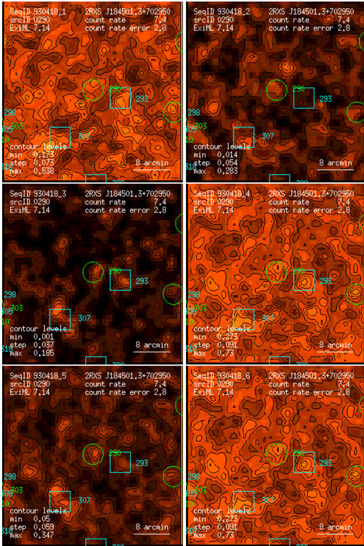
Figure 290: RASS 930418: detection 0290: band rate images, Gaussian filter: (1) PSPC channels 11 – 41, (2) 52 – 90, (3) 91 – 201, (4) 11 – 235, (5) 52 – 201, (6) 11 – 201. Broad band rates in counts/ks. Band rate contour levels in counts/ks/arcmin 2 .
