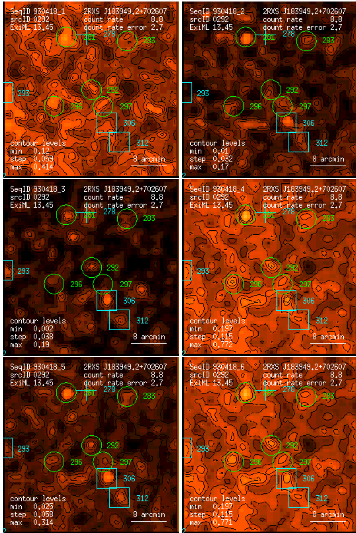
Figure 292: RASS 930418: detection 0292: band rate images, Gaussian filter: (1) PSPC channels 11 – 41, (2) 52 – 90, (3) 91 – 201, (4) 11 – 235, (5) 52 – 201, (6) 11 – 201. Broad band rates in counts/ks. Band rate contour levels in counts/ks/arcmin 2 .
