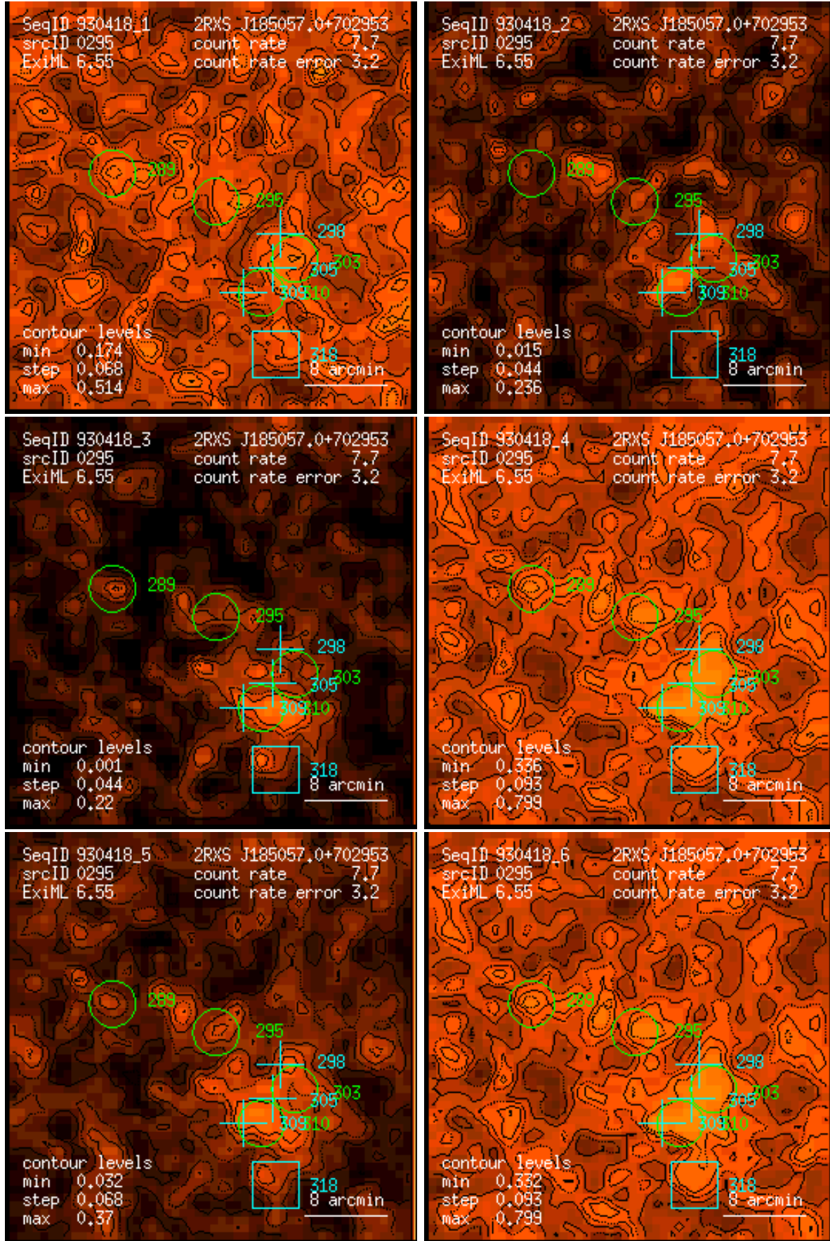
Figure 295: RASS 930418: detection 0295: band rate images, Gaussian filter: (1) PSPC channels 11 – 41, (2) 52 – 90, (3) 91 – 201, (4) 11 – 235, (5) 52 – 201, (6) 11 – 201. Broad band rates in counts/ks. Band rate contour levels in counts/ks/arcmin 2 .
