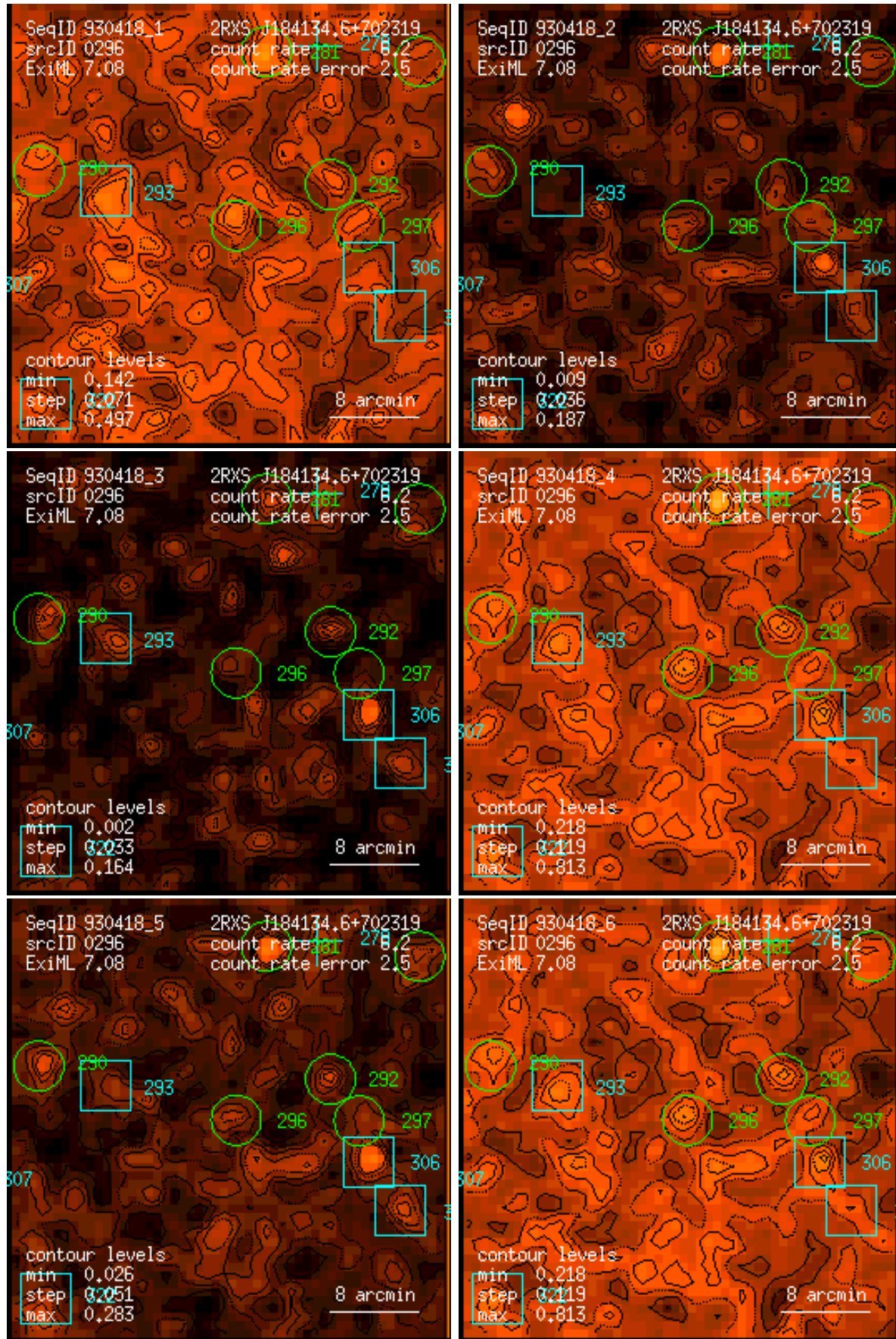
Figure 296: RASS 930418: detection 0296: band rate images, Gaussian filter: (1) PSPC channels 11 – 41, (2) 52 – 90, (3) 91 – 201, (4) 11 – 235, (5) 52 – 201, (6) 11 – 201. Broad band rates in counts/ks. Band rate contour levels in counts/ks/arcmin 2 .
