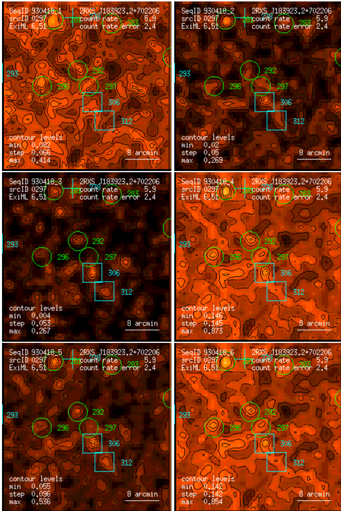
Figure 297: RASS 930418: detection 0297: band rate images, Gaussian filter: (1) PSPC channels 11 – 41, (2) 52 – 90, (3) 91 – 201, (4) 11 – 235, (5) 52 – 201, (6) 11 – 201. Broad band rates in counts/ks. Band rate contour levels in counts/ks/arcmin 2 .
