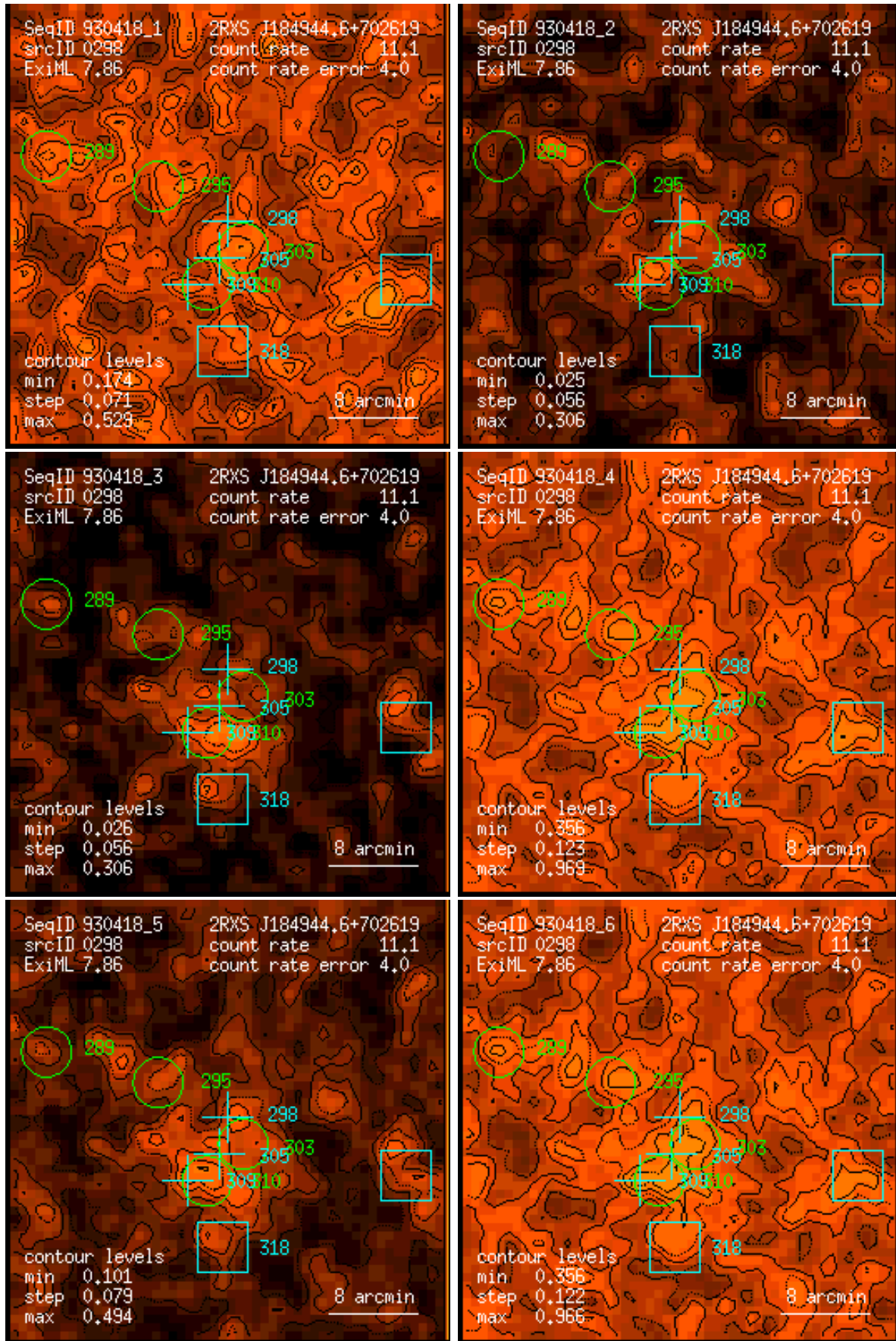
Figure 298: RASS 930418: detection 0298: band rate images, Gaussian filter: (1) PSPC channels 11 – 41, (2) 52 – 90, (3) 91 – 201, (4) 11 – 235, (5) 52 – 201, (6) 11 – 201. Broad band rates in counts/ks. Band rate contour levels in counts/ks/arcmin 2 .
