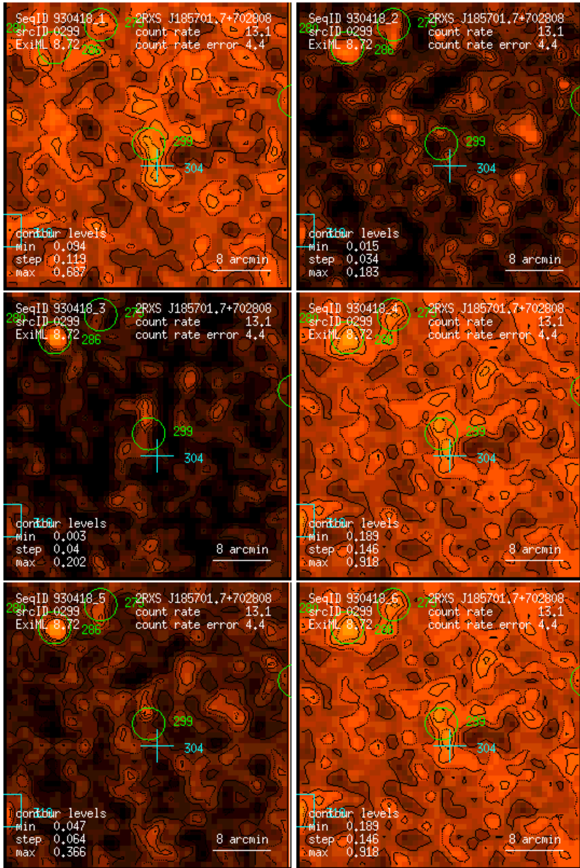
Figure 299: RASS 930418: detection 0299: band rate images, Gaussian filter: (1) PSPC channels 11 – 41, (2) 52 – 90, (3) 91 – 201, (4) 11 – 235, (5) 52 – 201, (6) 11 – 201. Broad band rates in counts/ks. Band rate contour levels in counts/ks/arcmin 2 .
