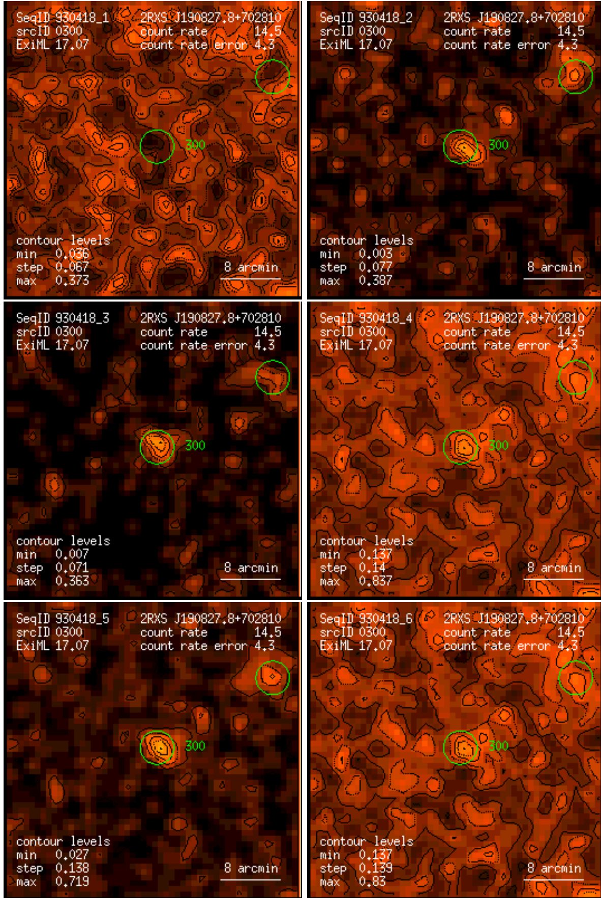
Figure 300: RASS 930418: detection 0300: band rate images, Gaussian filter: (1) PSPC channels 11 – 41, (2) 52 – 90, (3) 91 – 201, (4) 11 – 235, (5) 52 – 201, (6) 11 – 201. Broad band rates in counts/ks. Band rate contour levels in counts/ks/arcmin 2 .
