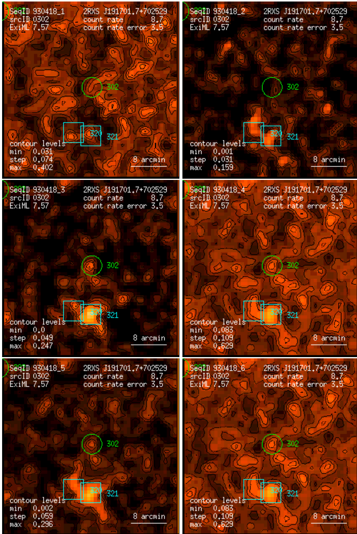
Figure 302: RASS 930418: detection 0302: band rate images, Gaussian filter: (1) PSPC channels 11 – 41, (2) 52 – 90, (3) 91 – 201, (4) 11 – 235, (5) 52 – 201, (6) 11 – 201. Broad band rates in counts/ks. Band rate contour levels in counts/ks/arcmin 2 .
