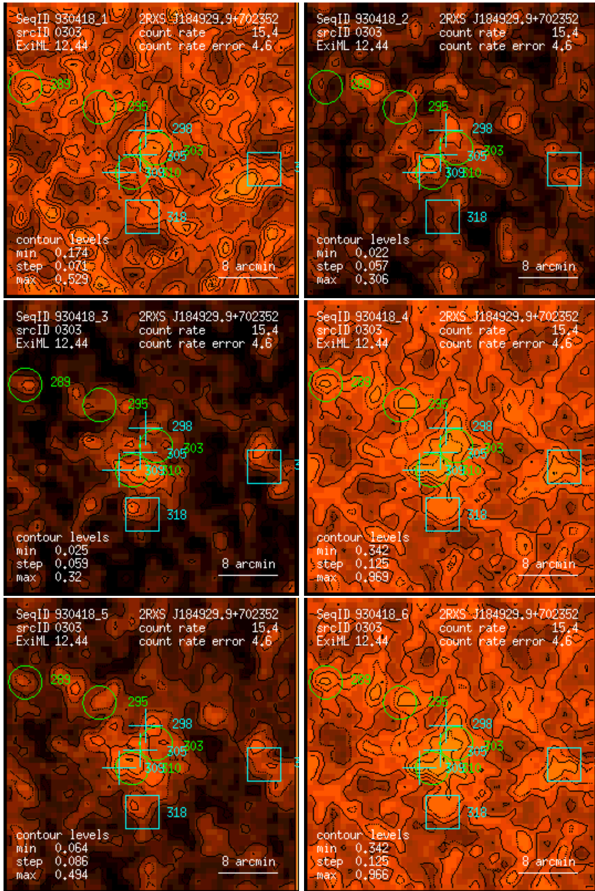
Figure 303: RASS 930418: detection 0303: band rate images, Gaussian filter: (1) PSPC channels 11 – 41, (2) 52 – 90, (3) 91 – 201, (4) 11 – 235, (5) 52 – 201, (6) 11 – 201. Broad band rates in counts/ks. Band rate contour levels in counts/ks/arcmin 2 .
