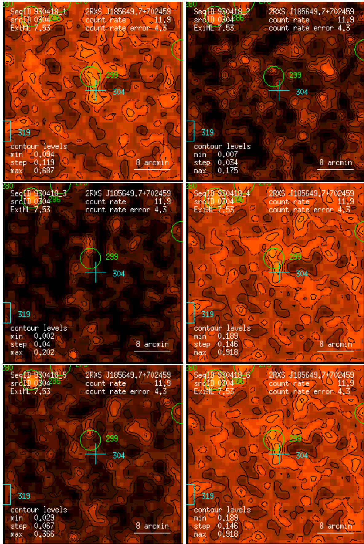
Figure 304: RASS 930418: detection 0304: band rate images, Gaussian filter: (1) PSPC channels 11 – 41, (2) 52 – 90, (3) 91 – 201, (4) 11 – 235, (5) 52 – 201, (6) 11 – 201. Broad band rates in counts/ks. Band rate contour levels in counts/ks/arcmin 2 .
