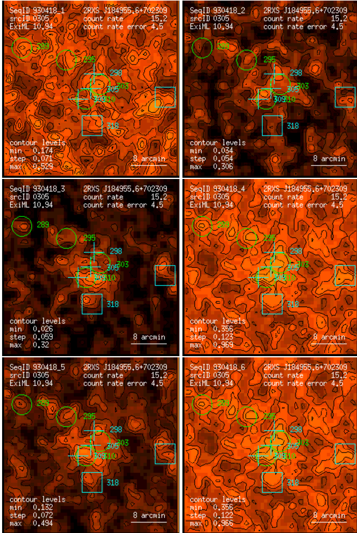
Figure 305: RASS 930418: detection 0305: band rate images, Gaussian filter: (1) PSPC channels 11 – 41, (2) 52 – 90, (3) 91 – 201, (4) 11 – 235, (5) 52 – 201, (6) 11 – 201. Broad band rates in counts/ks. Band rate contour levels in counts/ks/arcmin 2 .
