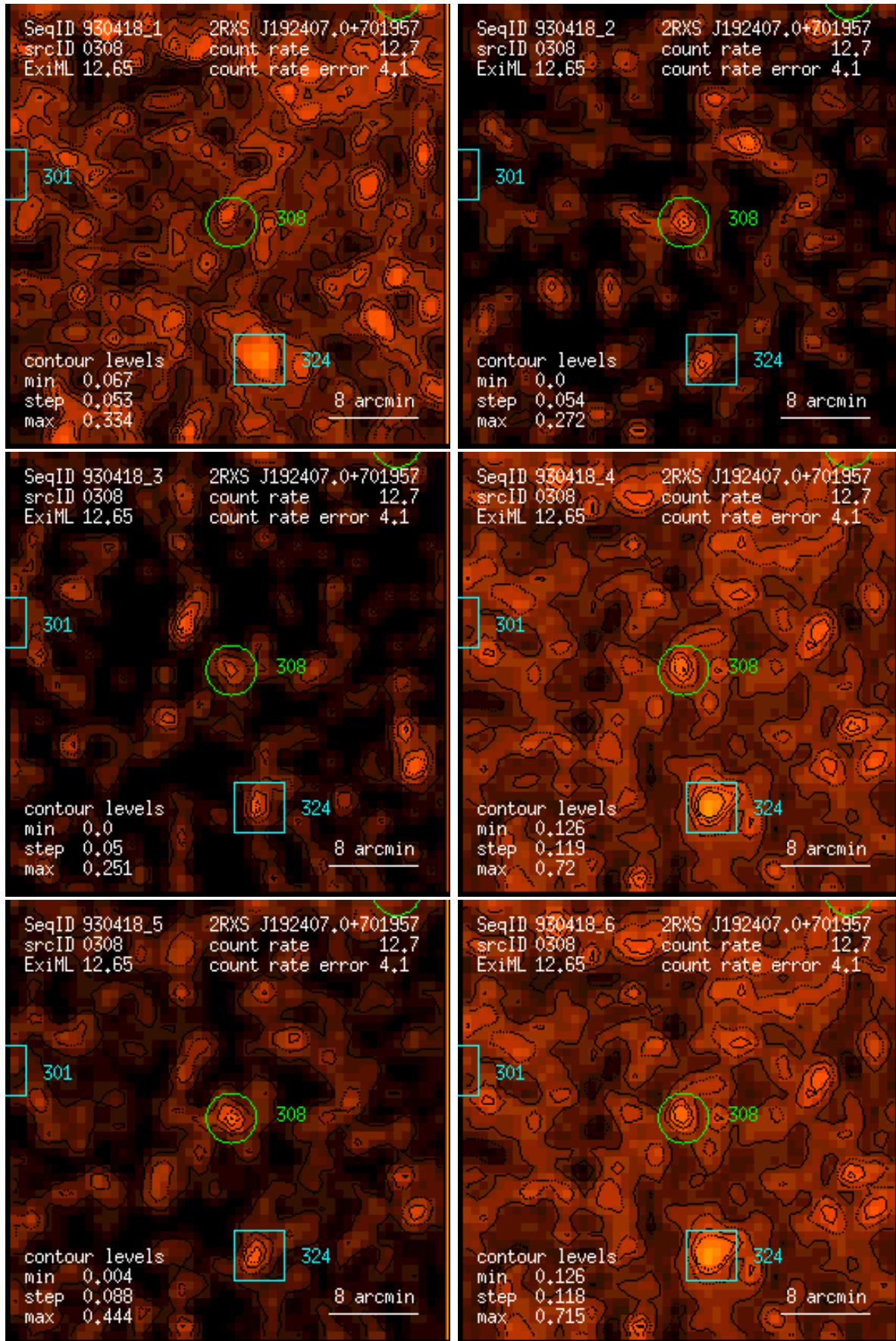
Figure 308: RASS 930418: detection 0308: band rate images, Gaussian filter: (1) PSPC channels 11 – 41, (2) 52 – 90, (3) 91 – 201, (4) 11 – 235, (5) 52 – 201, (6) 11 – 201. Broad band rates in counts/ks. Band rate contour levels in counts/ks/arcmin 2 .
