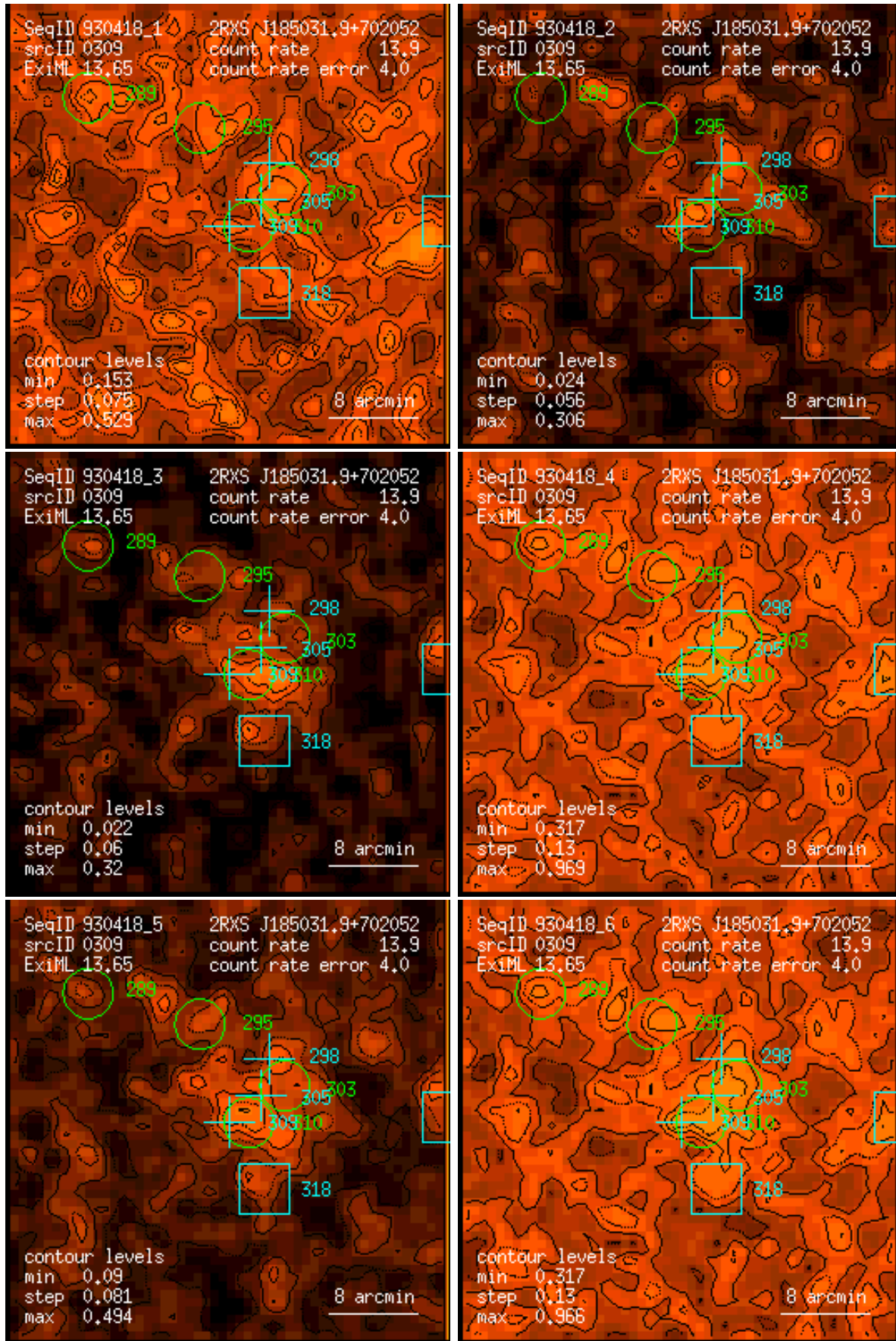
Figure 309: RASS 930418: detection 0309: band rate images, Gaussian filter: (1) PSPC channels 11 – 41, (2) 52 – 90, (3) 91 – 201, (4) 11 – 235, (5) 52 – 201, (6) 11 – 201. Broad band rates in counts/ks. Band rate contour levels in counts/ks/arcmin 2 .
