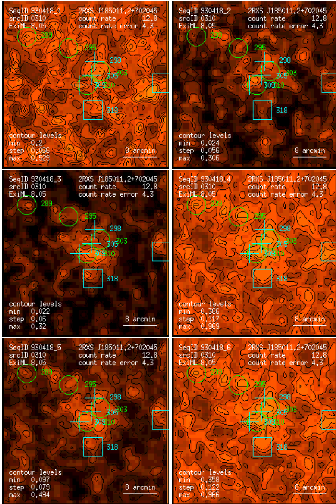
Figure 310: RASS 930418: detection 0310: band rate images, Gaussian filter: (1) PSPC channels 11 – 41, (2) 52 – 90, (3) 91 – 201, (4) 11 – 235, (5) 52 – 201, (6) 11 – 201. Broad band rates in counts/ks. Band rate contour levels in counts/ks/arcmin 2 .
