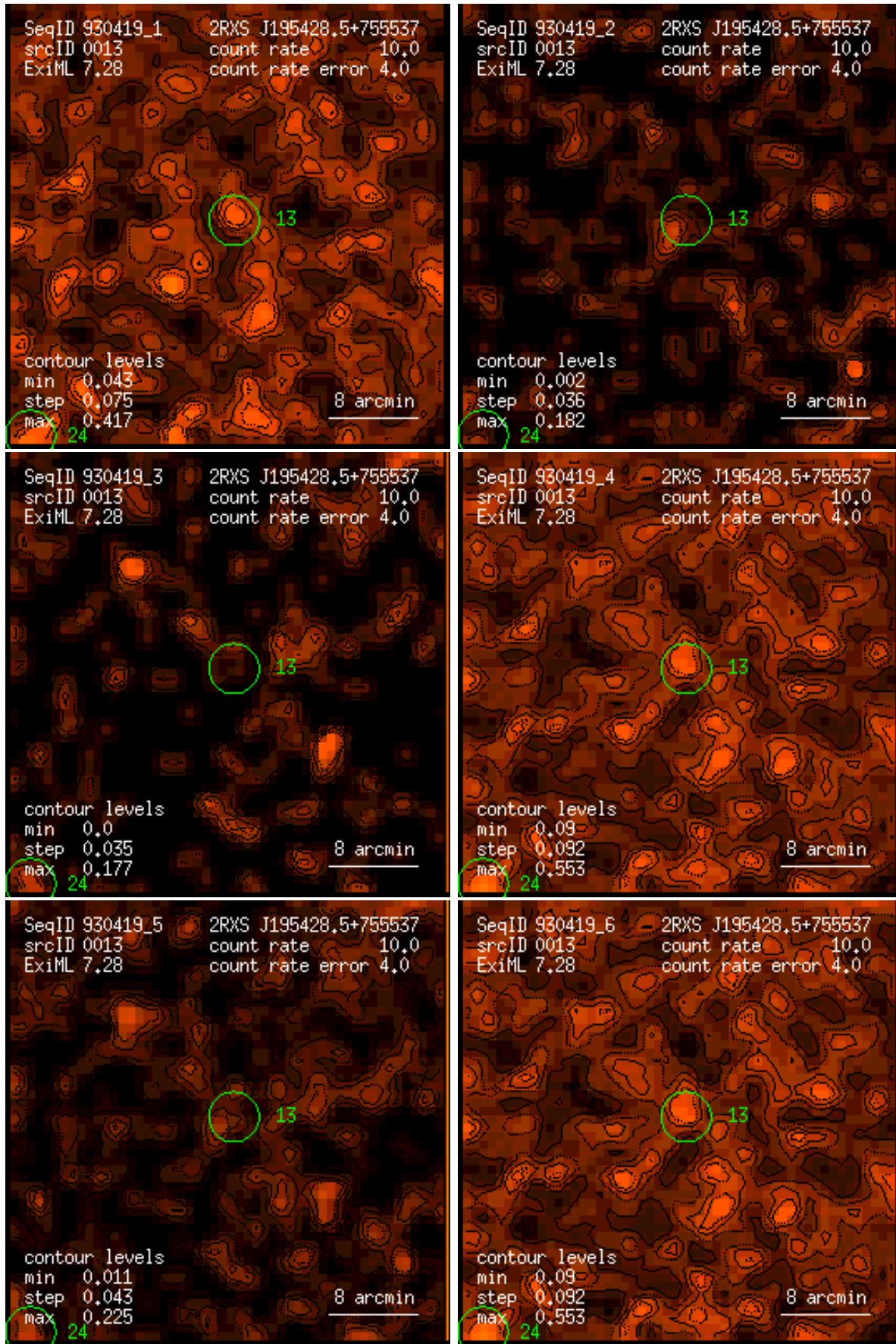
Figure 13: RASS 930419: detection 0013: band rate images, Gaussian filter: (1) PSPC channels 11 – 41, (2) 52 – 90, (3) 91 – 201, (4) 11 – 235, (5) 52 – 201, (6) 11 – 201. Broad band rates in counts/ks. Band rate contour levels in counts/ks/arcmin 2 .
