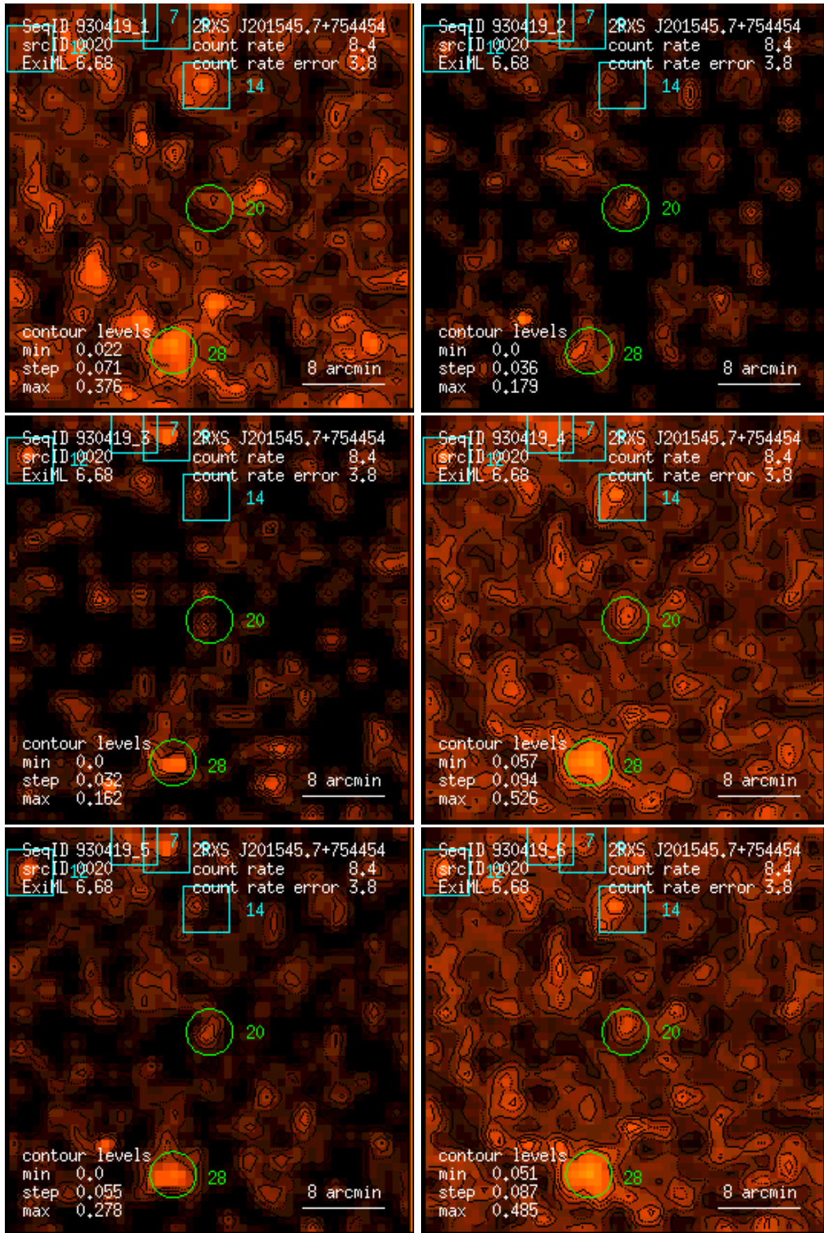
Figure 20: RASS 930419: detection 0020: band rate images, Gaussian filter: (1) PSPC channels 11 – 41, (2) 52 – 90, (3) 91 – 201, (4) 11 – 235, (5) 52 – 201, (6) 11 – 201. Broad band rates in counts/ks. Band rate contour levels in counts/ks/arcmin 2 .
