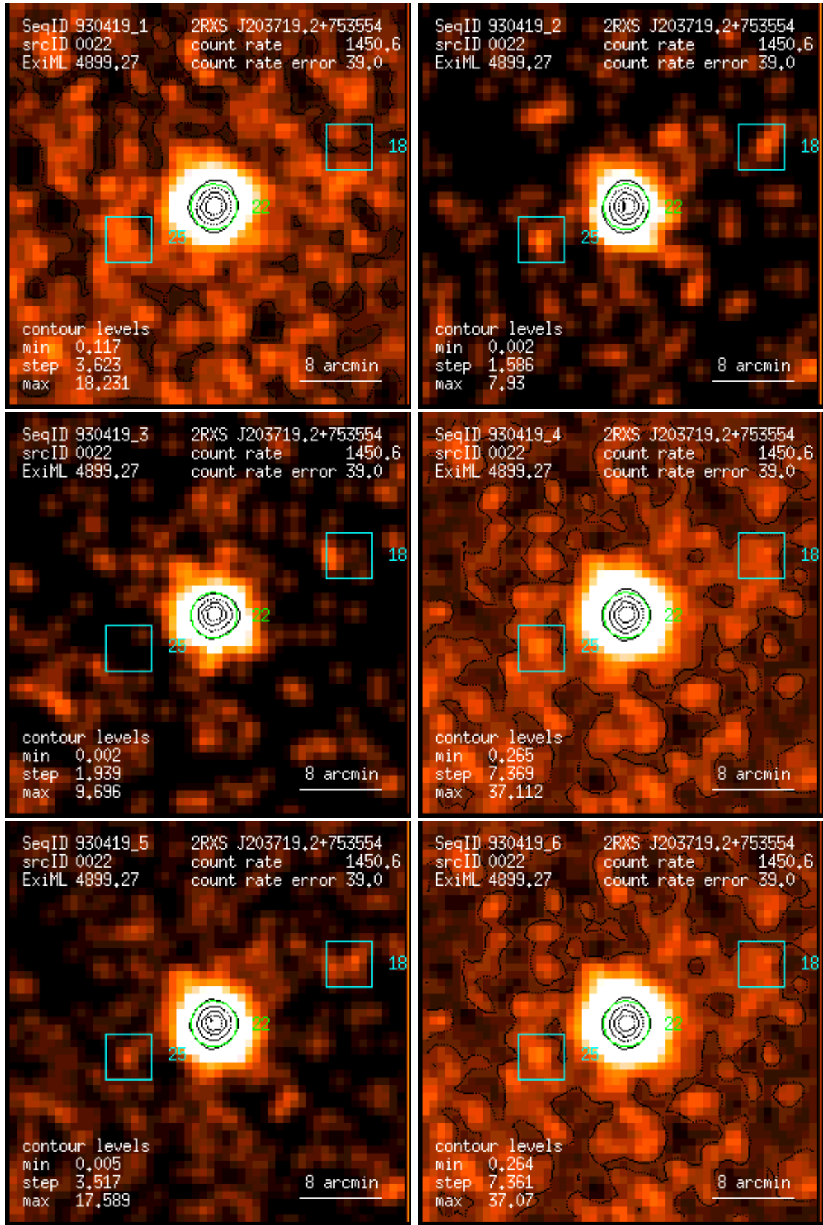
Figure 22: RASS 930419: detection 0022: band rate images, Gaussian filter: (1) PSPC channels 11 – 41, (2) 52 – 90, (3) 91 – 201, (4) 11 – 235, (5) 52 – 201, (6) 11 – 201. Broad band rates in counts/ks. Band rate contour levels in counts/ks/arcmin 2 .
