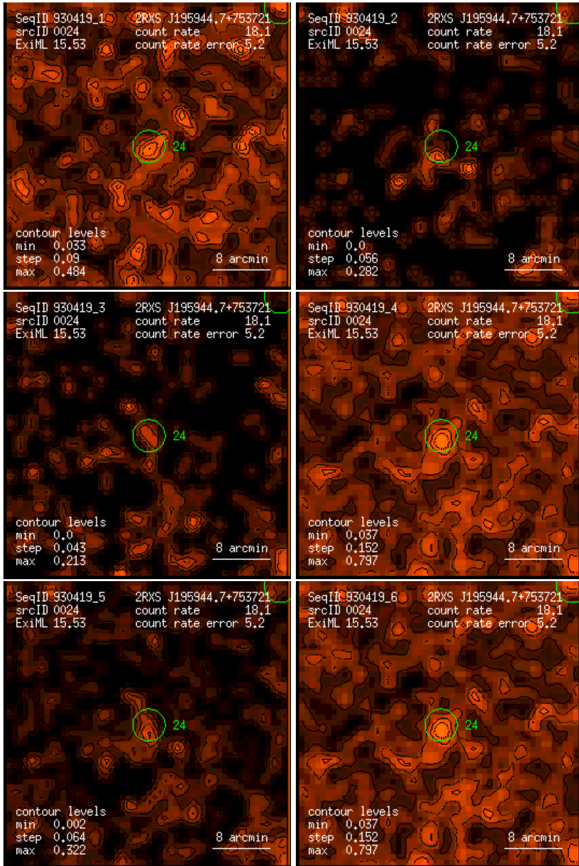
Figure 24: RASS 930419: detection 0024: band rate images, Gaussian filter: (1) PSPC channels 11 – 41, (2) 52 – 90, (3) 91 – 201, (4) 11 – 235, (5) 52 – 201, (6) 11 – 201. Broad band rates in counts/ks. Band rate contour levels in counts/ks/arcmin 2 .
