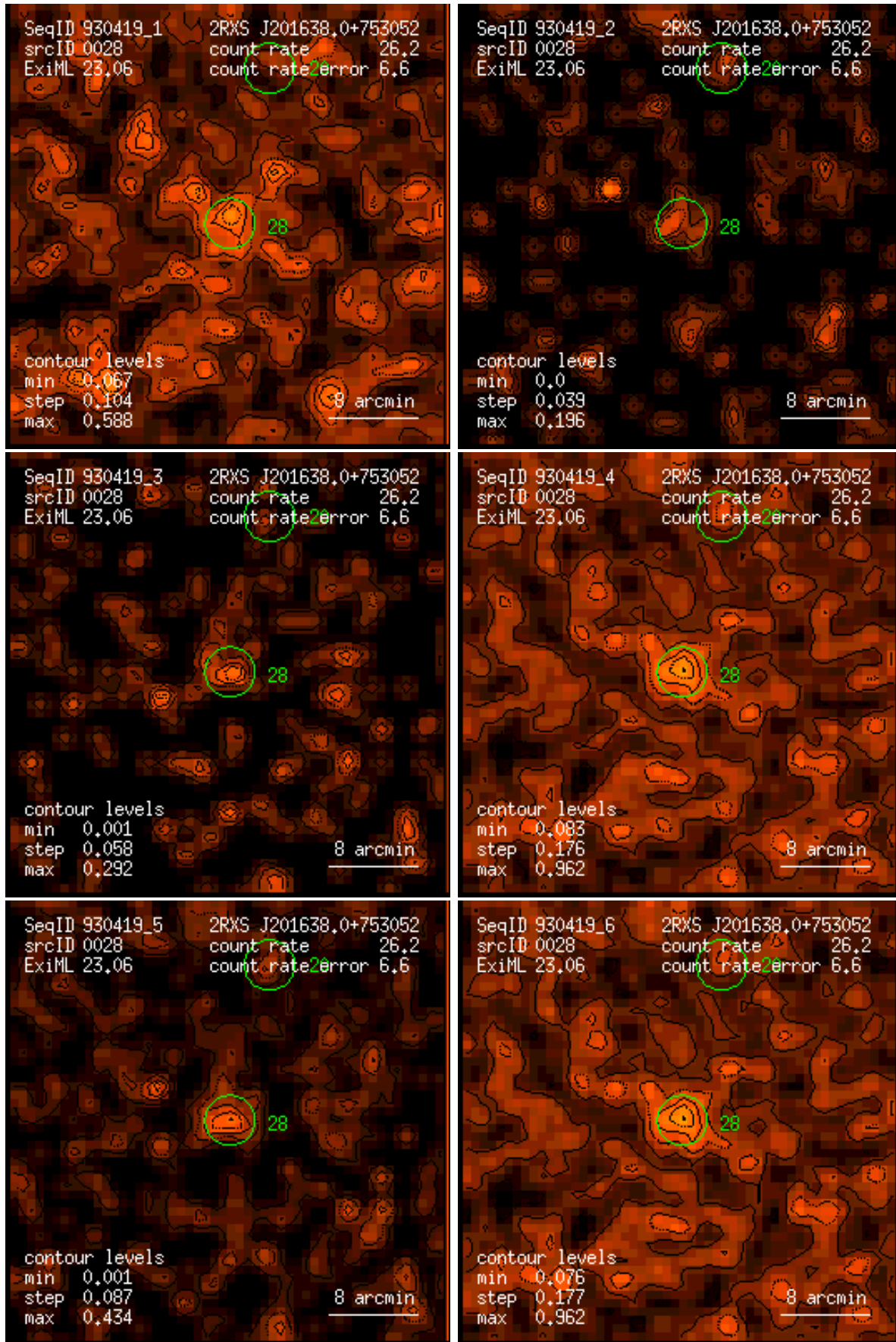
Figure 28: RASS 930419: detection 0028: band rate images, Gaussian filter: (1) PSPC channels 11 – 41, (2) 52 – 90, (3) 91 – 201, (4) 11 – 235, (5) 52 – 201, (6) 11 – 201. Broad band rates in counts/ks. Band rate contour levels in counts/ks/arcmin 2 .
