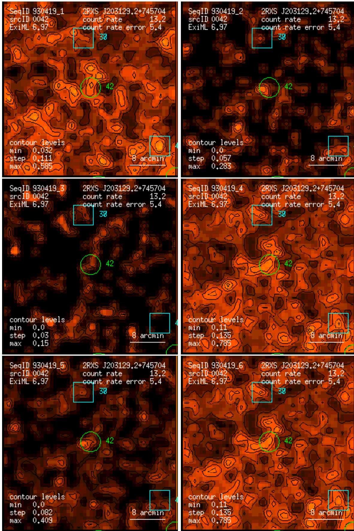
Figure 42: RASS 930419: detection 0042: band rate images, Gaussian filter: (1) PSPC channels 11 – 41, (2) 52 – 90, (3) 91 – 201, (4) 11 – 235, (5) 52 – 201, (6) 11 – 201. Broad band rates in counts/ks. Band rate contour levels in counts/ks/arcmin 2 .
