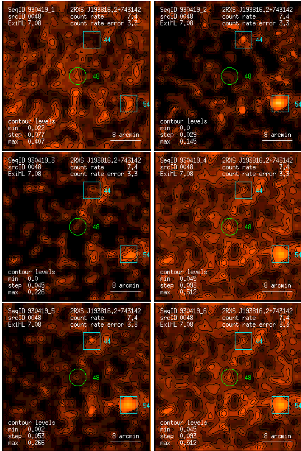
Figure 48: RASS 930419: detection 0048: band rate images, Gaussian filter: (1) PSPC channels 11 – 41, (2) 52 – 90, (3) 91 – 201, (4) 11 – 235, (5) 52 – 201, (6) 11 – 201. Broad band rates in counts/ks. Band rate contour levels in counts/ks/arcmin 2 .
