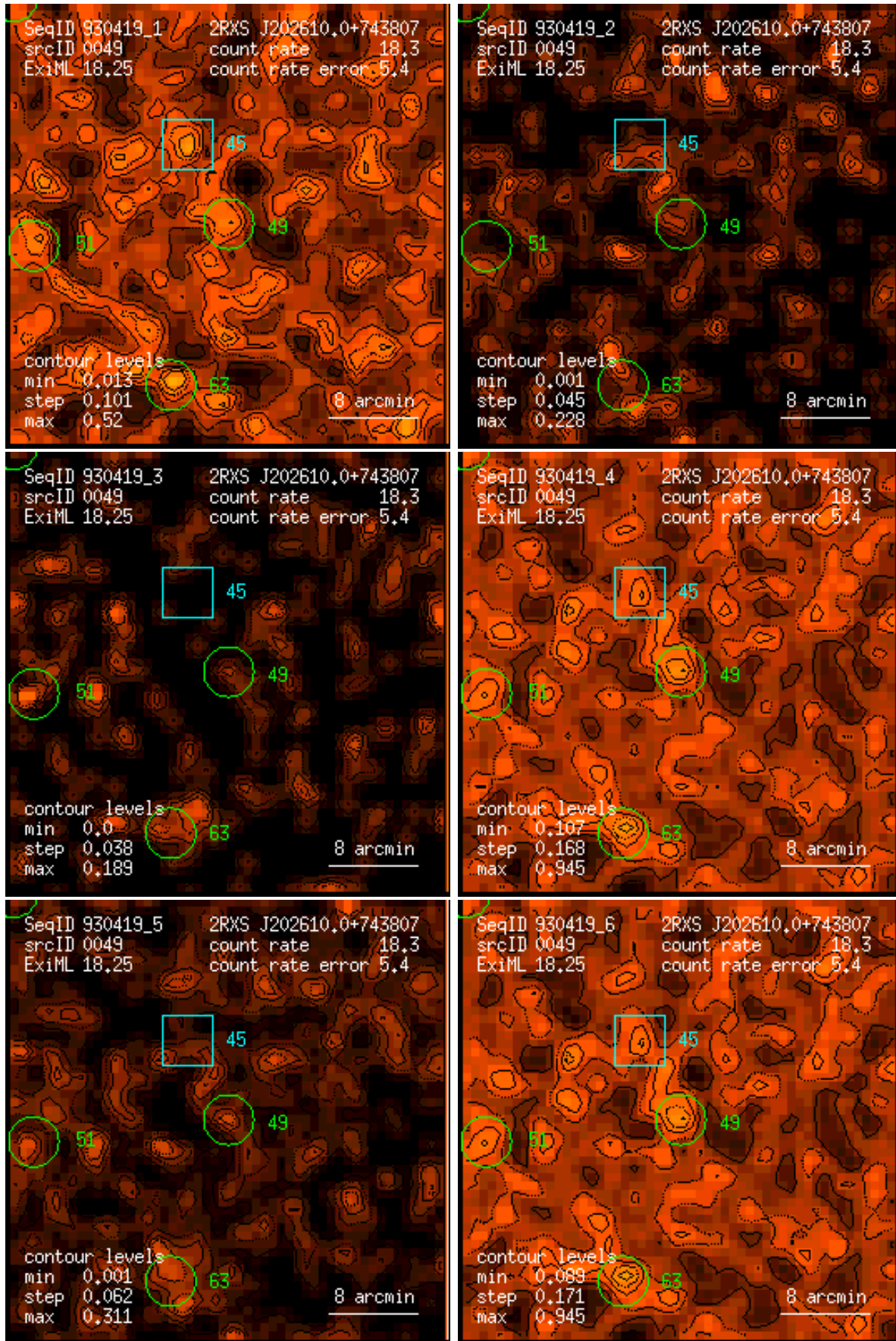
Figure 49: RASS 930419: detection 0049: band rate images, Gaussian filter: (1) PSPC channels 11 – 41, (2) 52 – 90, (3) 91 – 201, (4) 11 – 235, (5) 52 – 201, (6) 11 – 201. Broad band rates in counts/ks. Band rate contour levels in counts/ks/arcmin 2 .
