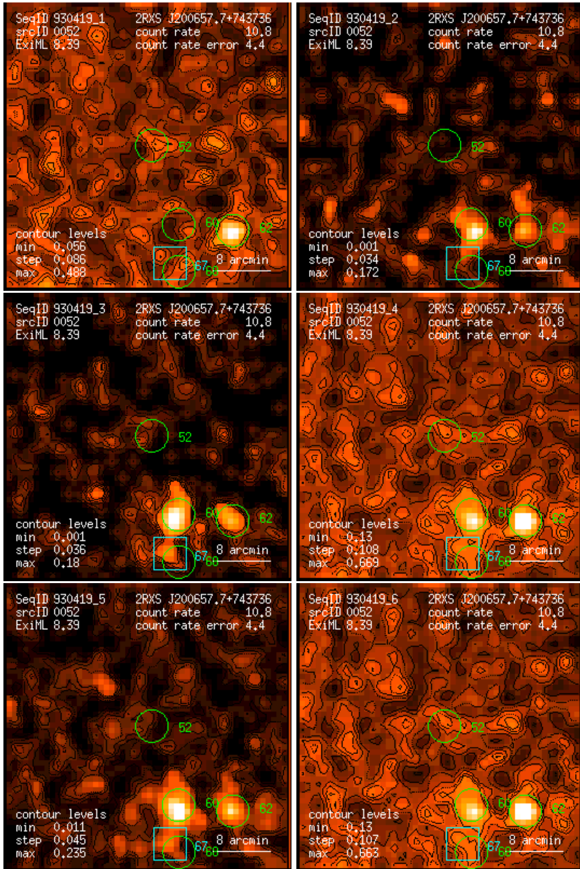
Figure 52: RASS 930419: detection 0052: band rate images, Gaussian filter: (1) PSPC channels 11 – 41, (2) 52 – 90, (3) 91 – 201, (4) 11 – 235, (5) 52 – 201, (6) 11 – 201. Broad band rates in counts/ks. Band rate contour levels in counts/ks/arcmin 2 .
