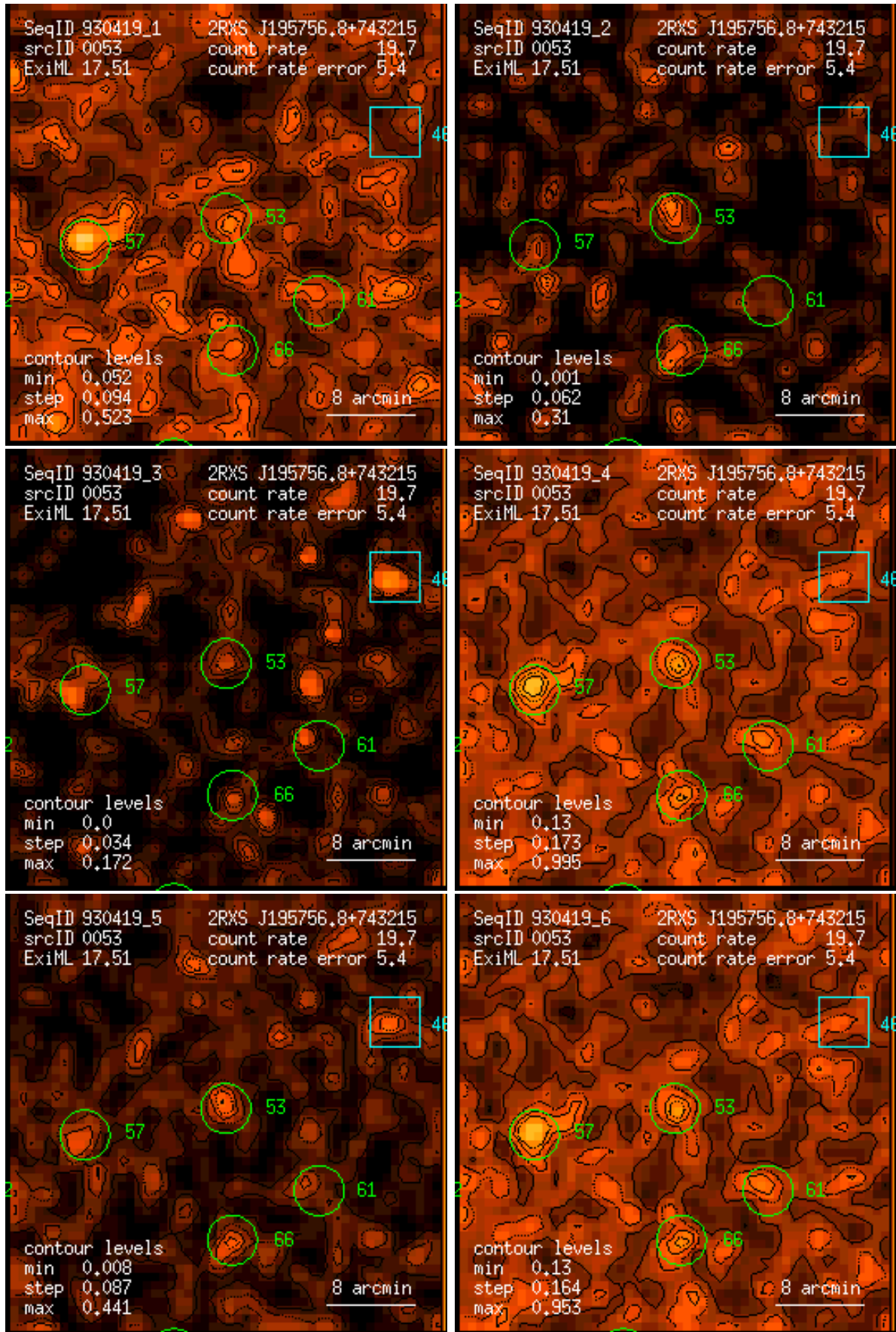
Figure 53: RASS 930419: detection 0053: band rate images, Gaussian filter: (1) PSPC channels 11 – 41, (2) 52 – 90, (3) 91 – 201, (4) 11 – 235, (5) 52 – 201, (6) 11 – 201. Broad band rates in counts/ks. Band rate contour levels in counts/ks/arcmin 2 .
