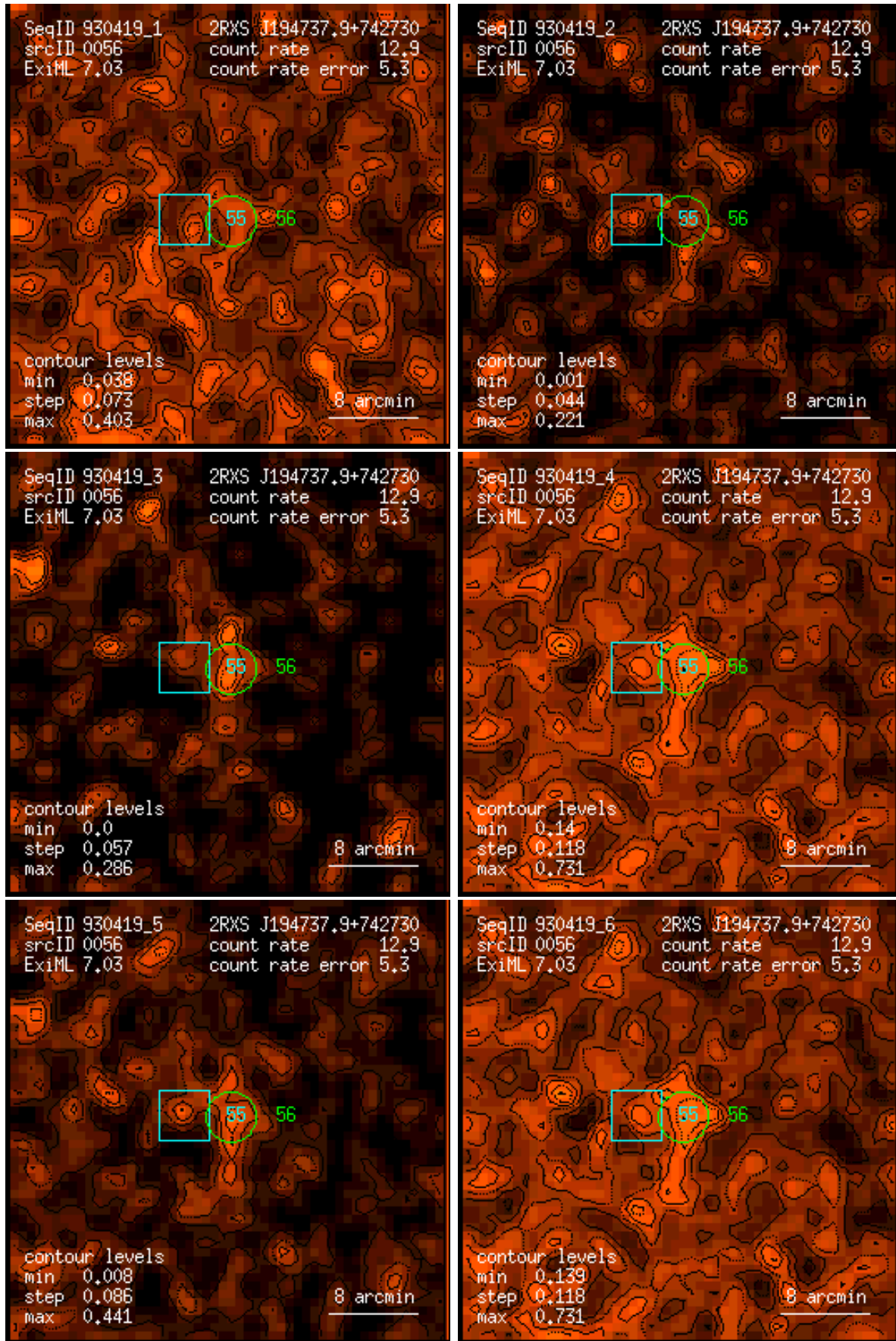
Figure 56: RASS 930419: detection 0056: band rate images, Gaussian filter: (1) PSPC channels 11 – 41, (2) 52 – 90, (3) 91 – 201, (4) 11 – 235, (5) 52 – 201, (6) 11 – 201. Broad band rates in counts/ks. Band rate contour levels in counts/ks/arcmin 2 .
