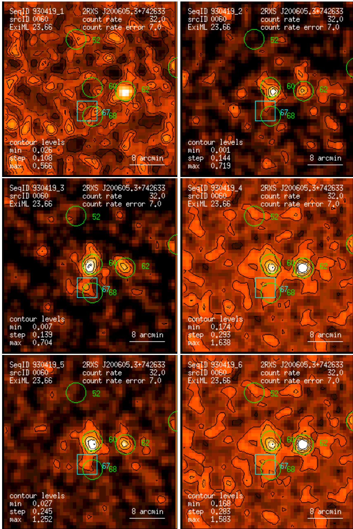
Figure 60: RASS 930419: detection 0060: band rate images, Gaussian filter: (1) PSPC channels 11 – 41, (2) 52 – 90, (3) 91 – 201, (4) 11 – 235, (5) 52 – 201, (6) 11 – 201. Broad band rates in counts/ks. Band rate contour levels in counts/ks/arcmin 2 .
