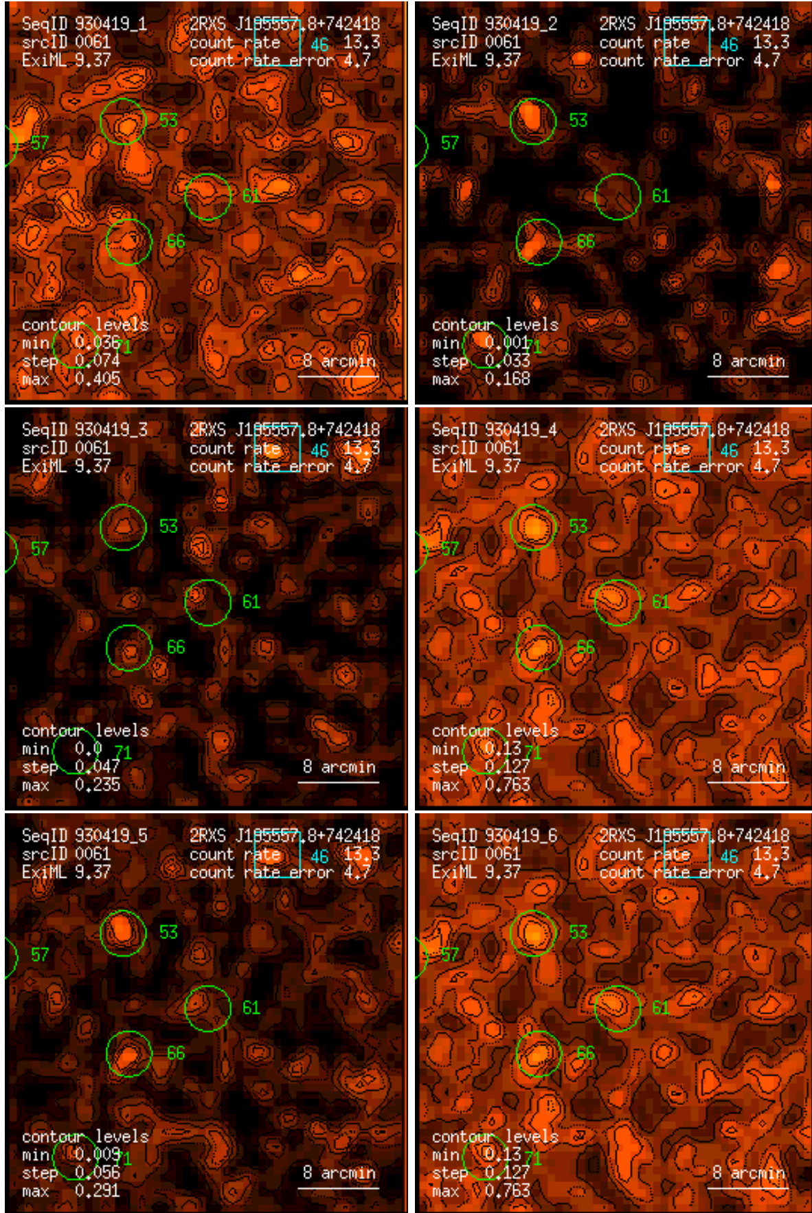
Figure 61: RASS 930419: detection 0061: band rate images, Gaussian filter: (1) PSPC channels 11 – 41, (2) 52 – 90, (3) 91 – 201, (4) 11 – 235, (5) 52 – 201, (6) 11 – 201. Broad band rates in counts/ks. Band rate contour levels in counts/ks/arcmin 2 .
