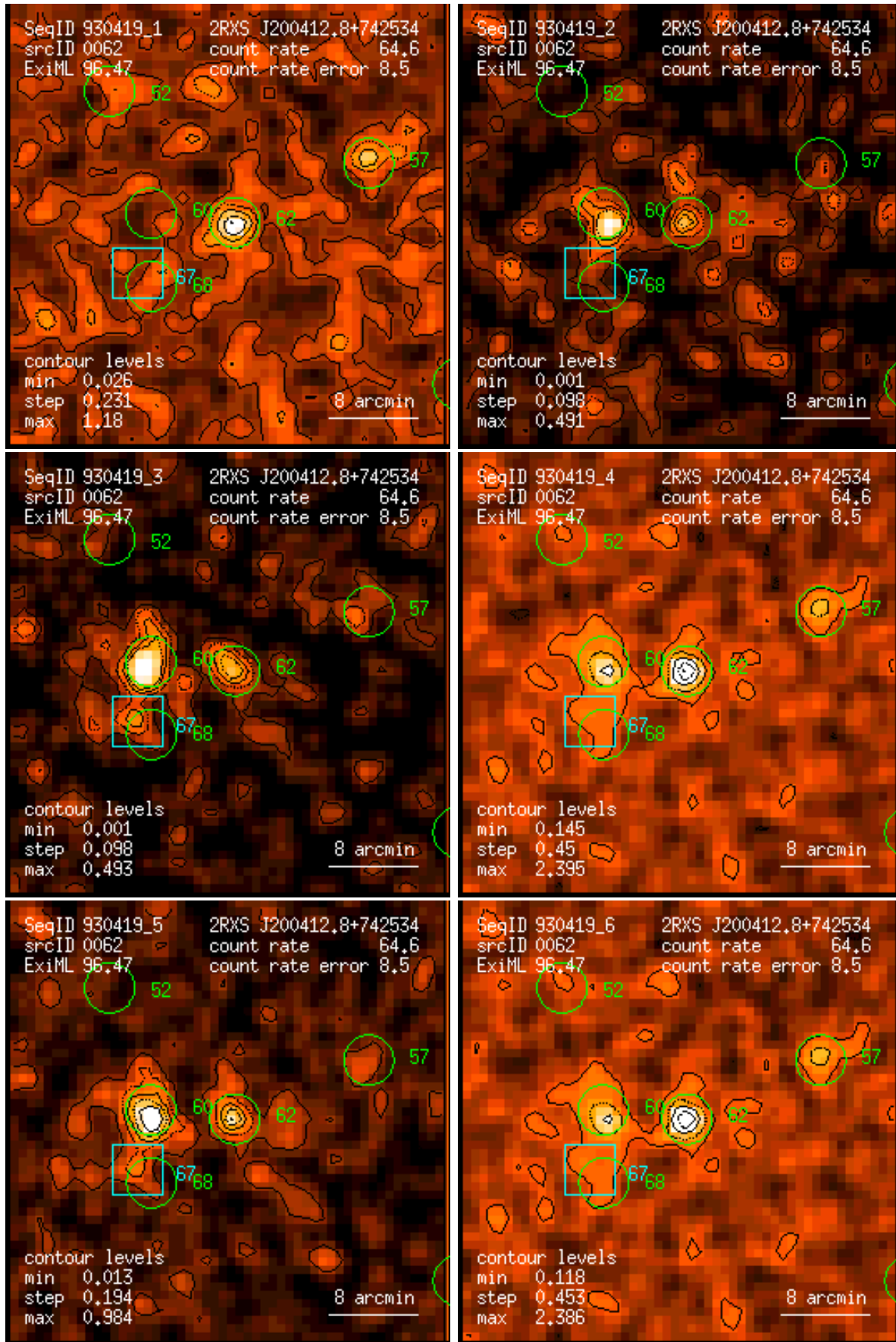
Figure 62: RASS 930419: detection 0062: band rate images, Gaussian filter: (1) PSPC channels 11 – 41, (2) 52 – 90, (3) 91 – 201, (4) 11 – 235, (5) 52 – 201, (6) 11 – 201. Broad band rates in counts/ks. Band rate contour levels in counts/ks/arcmin 2 .
