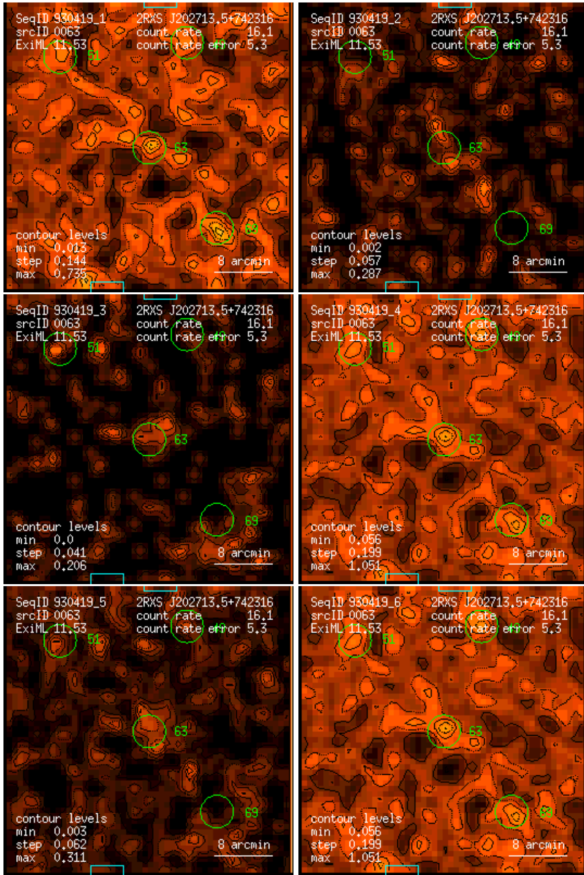
Figure 63: RASS 930419: detection 0063: band rate images, Gaussian filter: (1) PSPC channels 11 – 41, (2) 52 – 90, (3) 91 – 201, (4) 11 – 235, (5) 52 – 201, (6) 11 – 201. Broad band rates in counts/ks. Band rate contour levels in counts/ks/arcmin 2 .
