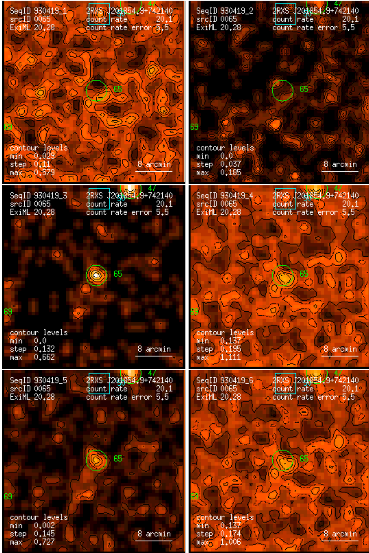
Figure 65: RASS 930419: detection 0065: band rate images, Gaussian filter: (1) PSPC channels 11 – 41, (2) 52 – 90, (3) 91 – 201, (4) 11 – 235, (5) 52 – 201, (6) 11 – 201. Broad band rates in counts/ks. Band rate contour levels in counts/ks/arcmin 2 .
