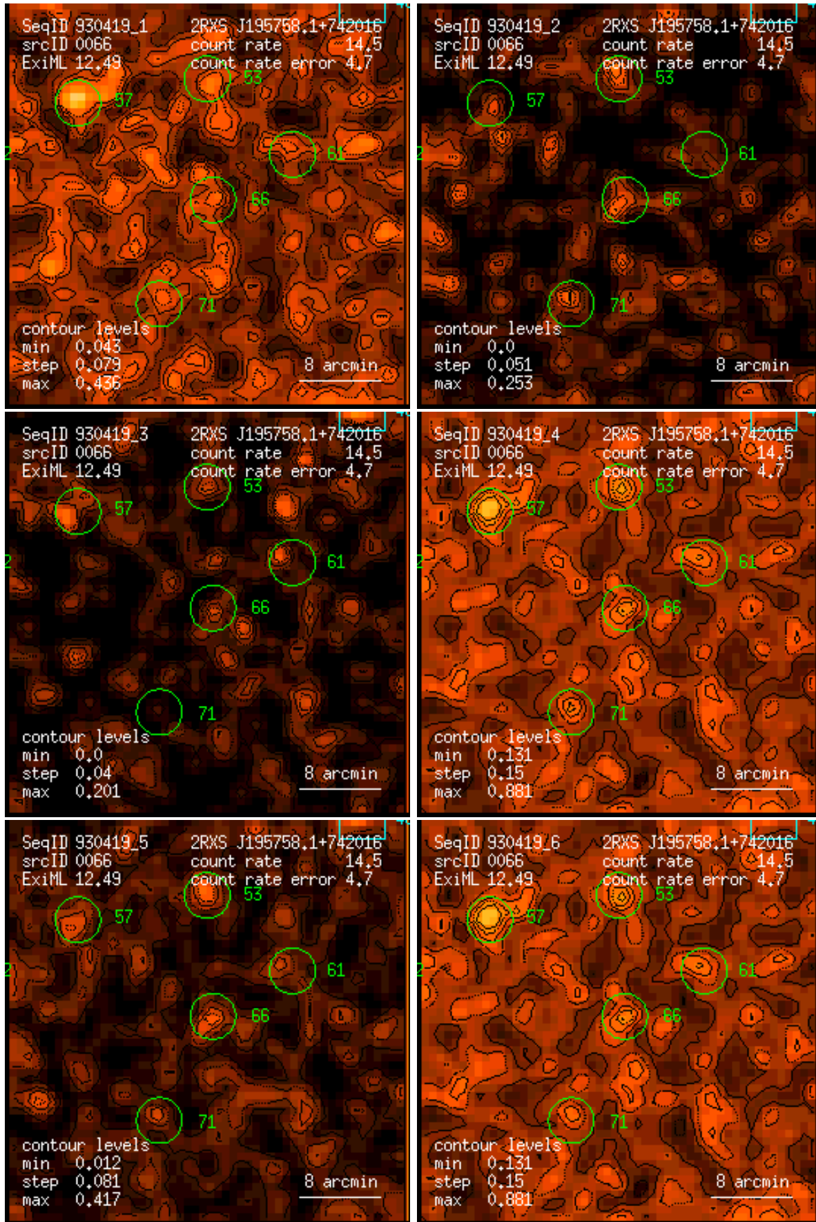
Figure 66: RASS 930419: detection 0066: band rate images, Gaussian filter: (1) PSPC channels 11 – 41, (2) 52 – 90, (3) 91 – 201, (4) 11 – 235, (5) 52 – 201, (6) 11 – 201. Broad band rates in counts/ks. Band rate contour levels in counts/ks/arcmin 2 .
